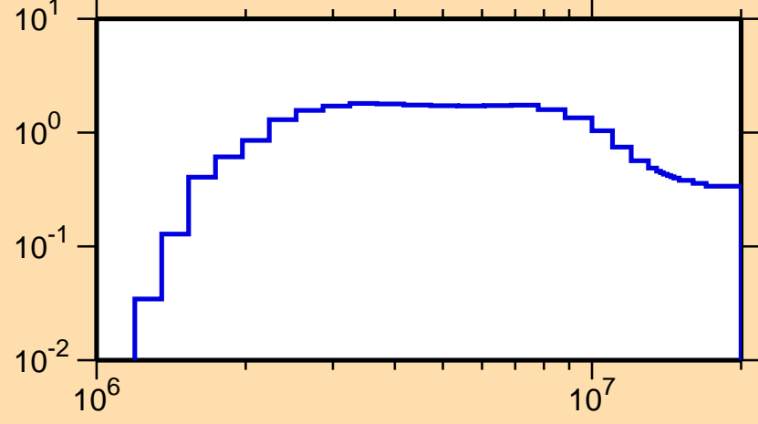
\sigma vs. E for ^{91}\text{Zr}(n,\text{inel.})
