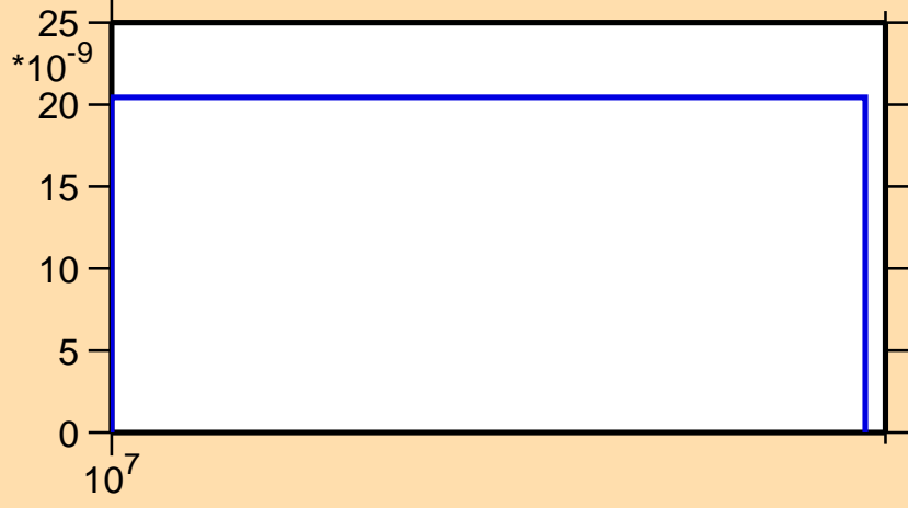
\sigma vs. E for ^{91}\text{Zr}(n,\text{He}3)
