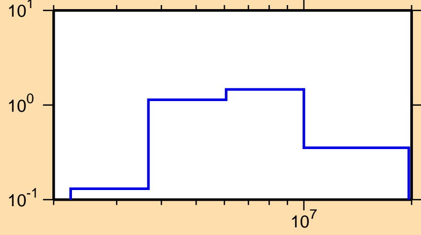
\sigma vs. E for ^{91}\text{Zr}(n,n\text{cont.})
