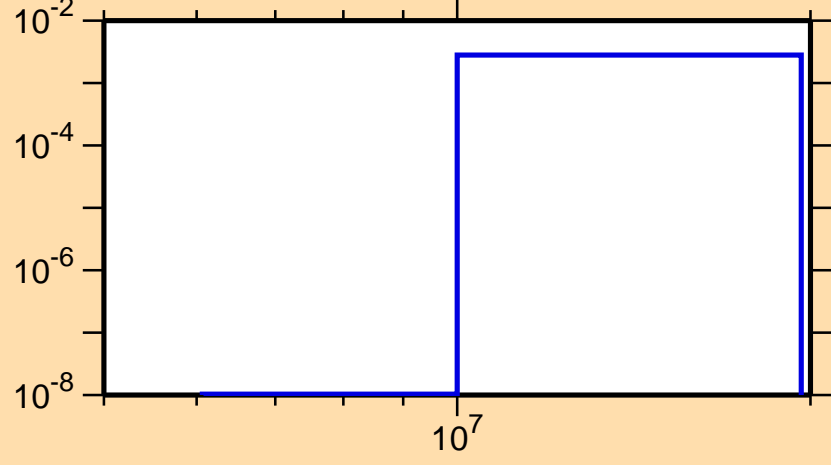
\sigma vs. E for ^{91}\text{Zr}(n,d)
