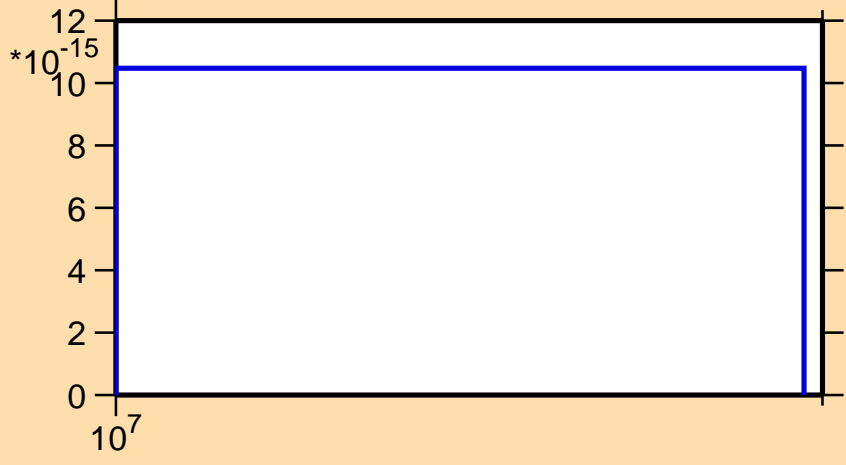
\sigma vs. E for ^{91}\text{Zr}(n,pd)
