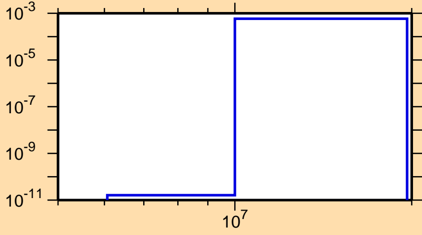
\sigma vs. E for ^{91}\text{Zr}(n,t)
