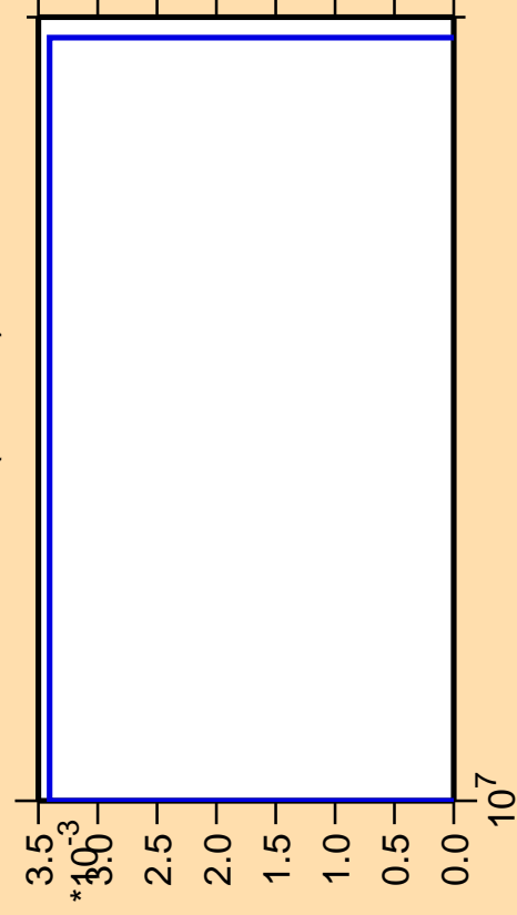
\Delta\sigma/\sigma vs. E for ^{91}\text{Zr}(\text{mt } 34)
