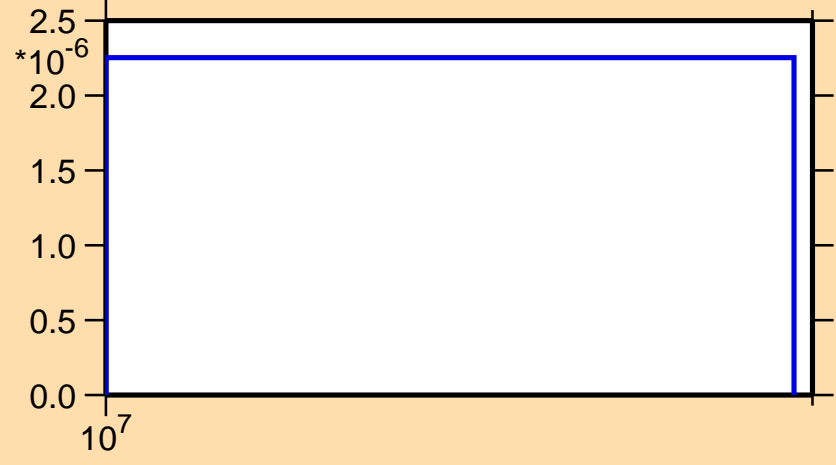
\sigma vs. E for ^{91}\text{Zr}(n,2np)
