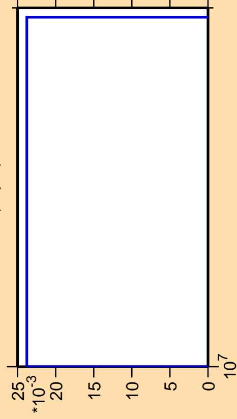
\Delta\sigma/\sigma vs. E for ^{91}\text{Zr}(n,pd)
