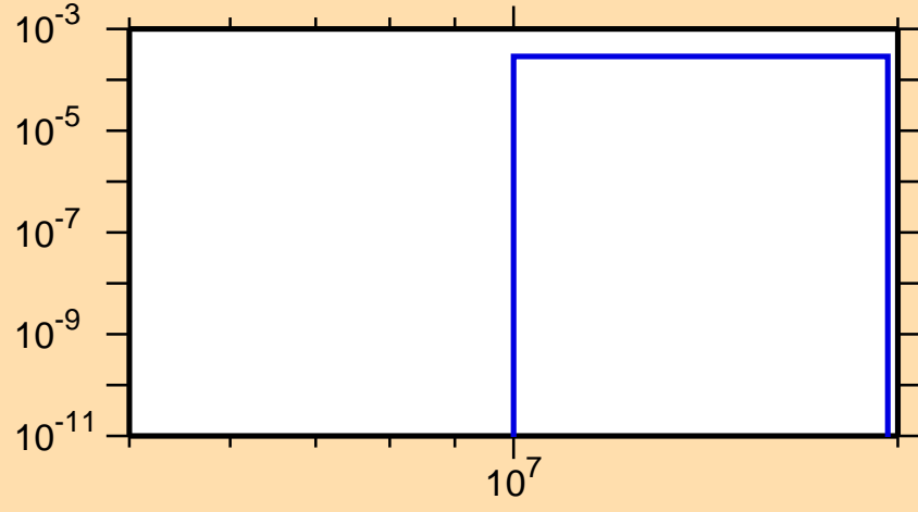
\sigma vs. E for ^{91}\text{Zr}(n,n\alpha)
