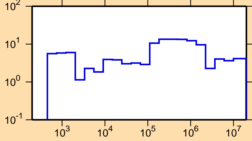
\Delta\sigma/\sigma vs. E for ^{92}\text{Zr}(n,\text{tot.})
