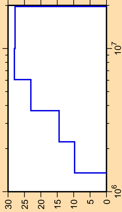
\Delta\sigma/\sigma vs. E for ^{92}\text{Zr}(n,n_4)
