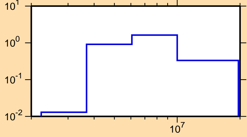
\sigma vs. E for ^{92}\text{Zr}(n,n\text{cont.})
