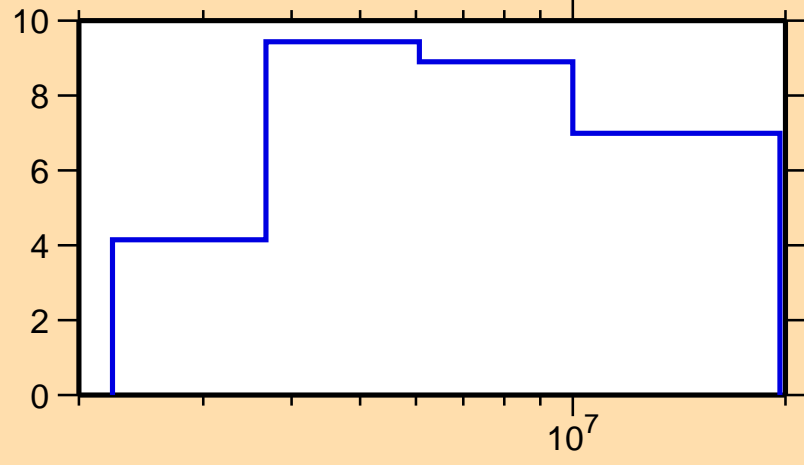
\Delta\sigma/\sigma vs. E for ^{92}\text{Zr}(n,el.)
