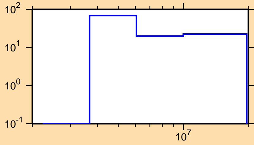
\Delta\sigma/\sigma vs. E for ^{92}\text{Zr}(n,p)
