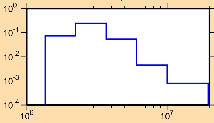
\sigma vs. E for ^{92}\text{Zr}(n,n_4)
