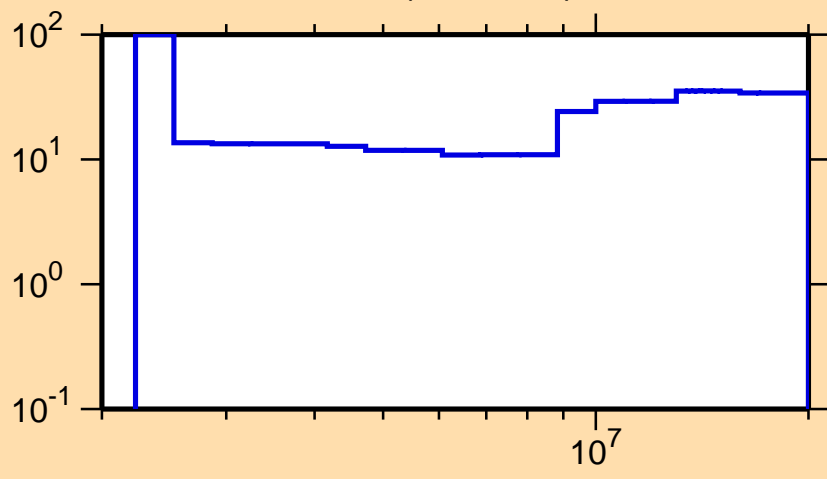
\Delta\sigma/\sigma vs. E for ^{93}\text{Zr}(n,n\text{cont.})
