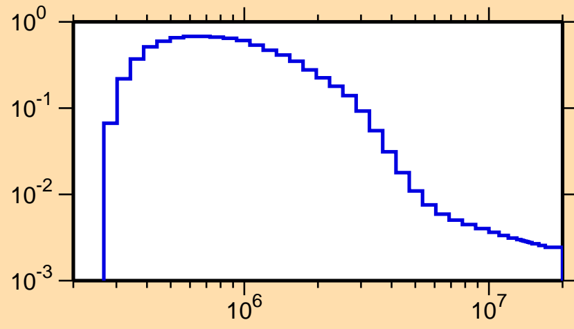
\sigma vs. E for ^{93}\text{Zr}(n,n_1)
