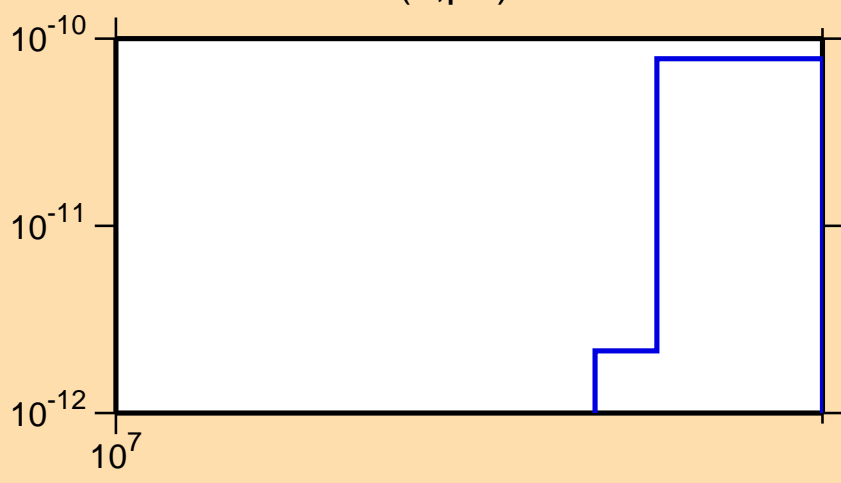
\sigma vs. E for ^{93}\text{Zr}(n,p\alpha)
