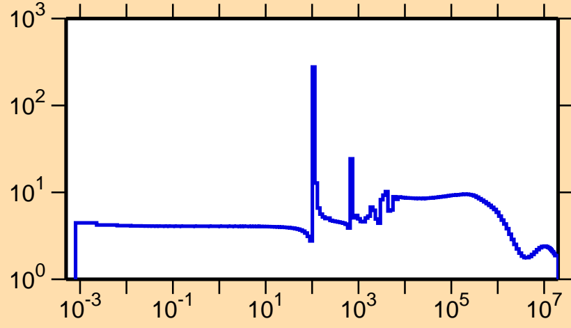
\sigma vs. E for ^{93}\text{Zr}(n,\text{el.})
