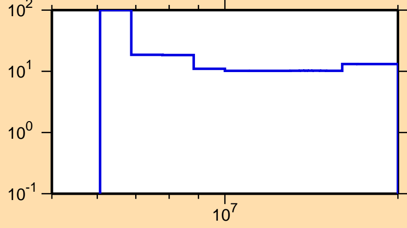
\Delta\sigma/\sigma vs. E for ^{93}\text{Zr}(n,2n)
