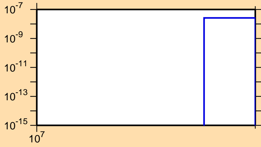
\sigma vs. E for ^{93}\text{Zr}(n,nt)
