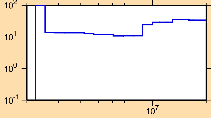
\Delta\sigma/\sigma vs. E for ^{93}\text{Zr}(n,n\text{cont.})
