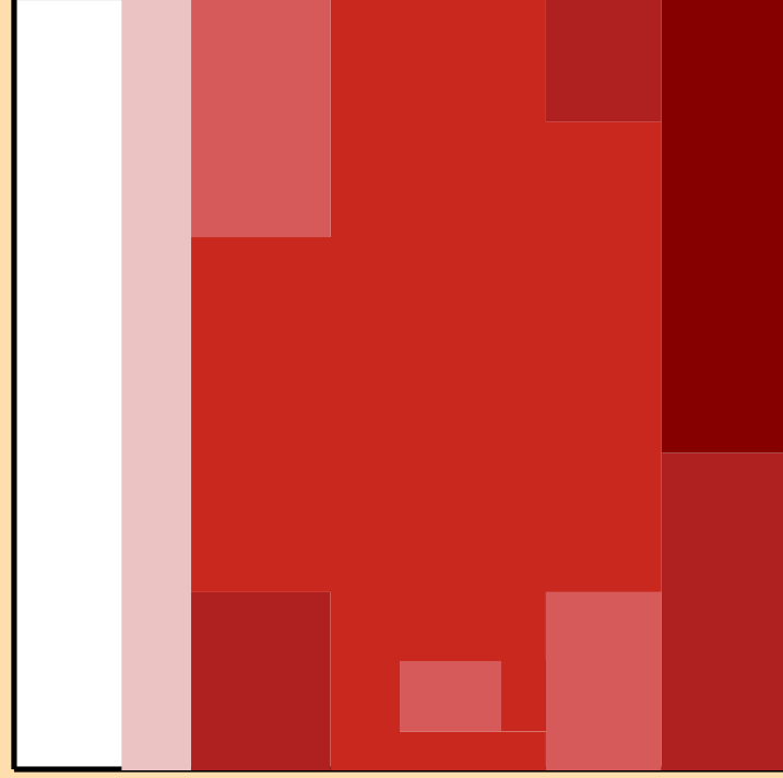
\Delta\sigma/\sigma vs. E for ^{93}\text{Zr}(n,2n)
