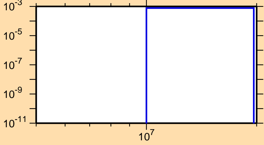
\sigma vs. E for ^{93}\text{Zr}(n,np)
