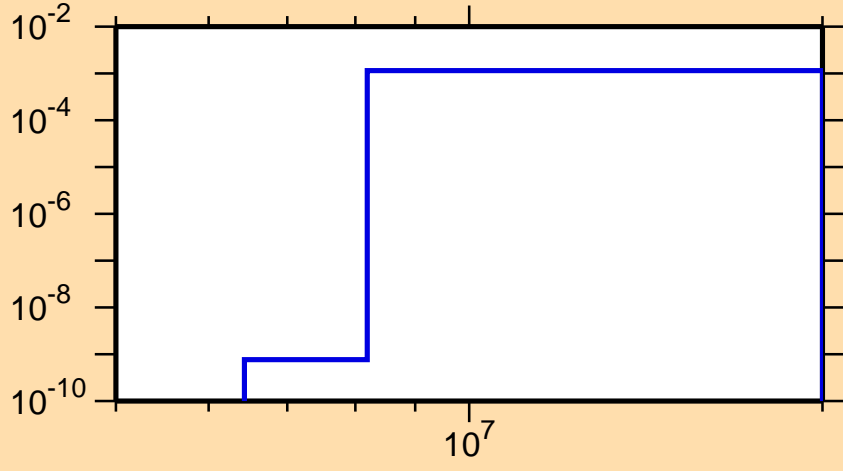
\sigma vs. E for ^{93}\text{Zr}(n,n\alpha)
