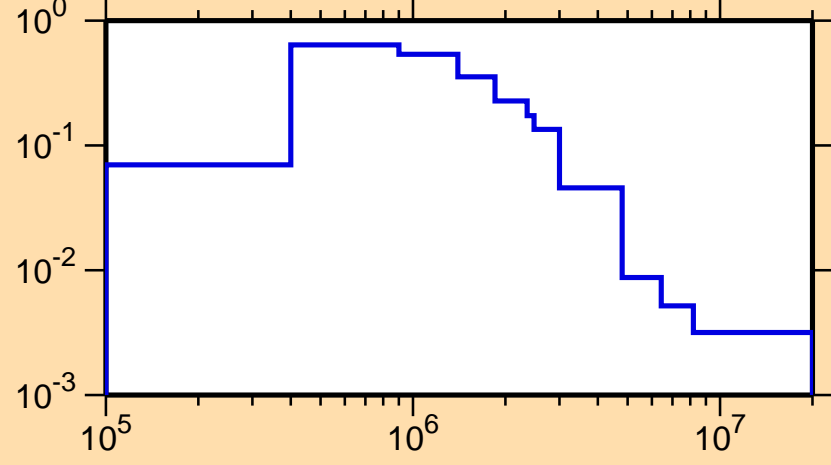
\sigma vs. E for ^{93}\text{Zr}(n,n_1)
