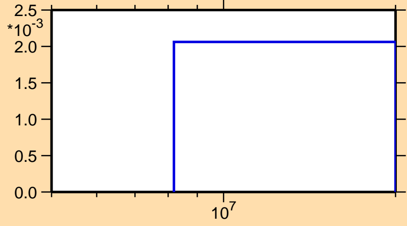
\sigma vs. E for ^{93}\text{Zr}(n,3n)
