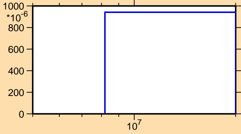
\sigma vs. E for ^{93}\text{Zr}(n,d)
