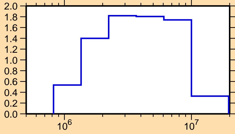
\sigma vs. E for ^{94}\text{Zr}(n,\text{inel.})
