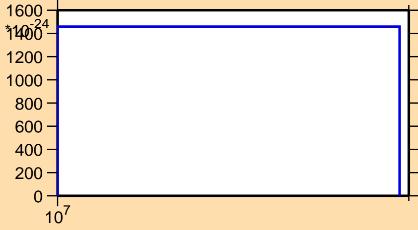
\sigma vs. E for ^{94}\text{Zr}(n,3n\alpha)
