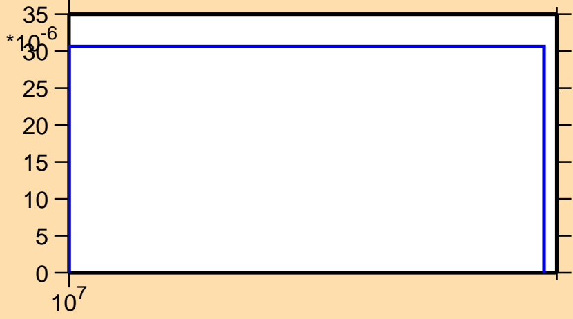
\sigma vs. E for ^{94}\text{Zr}(n,t)
