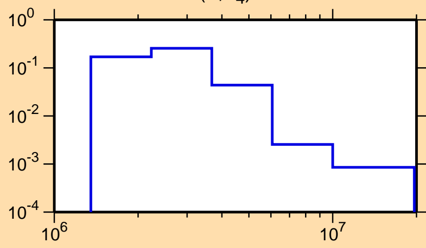
\sigma vs. E for ^{94}\text{Zr}(n,n_4)
