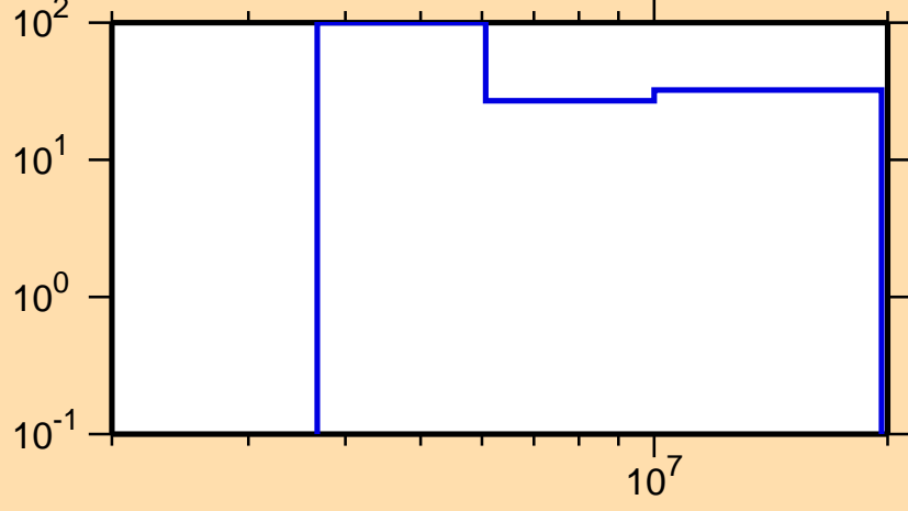
\Delta\sigma/\sigma vs. E for ^{94}\text{Zr}(n,p)
