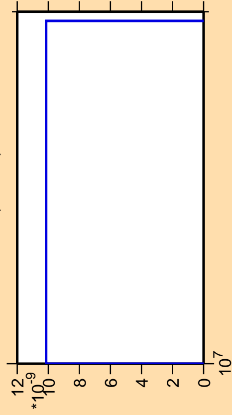
\Delta\sigma/\sigma vs. E for ^{94}\text{Zr}(\text{mt } 34)
