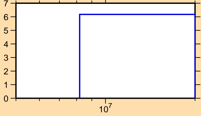
\Delta\sigma/\sigma vs. E for ^{94}\text{Zr}(n,\text{el.})
