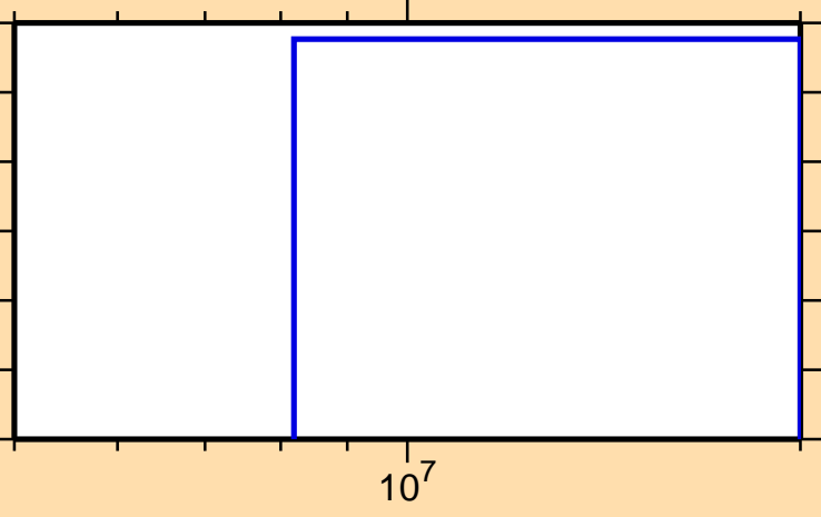
\sigma vs. E for ^{94}\text{Zr}(n,2n\alpha)
