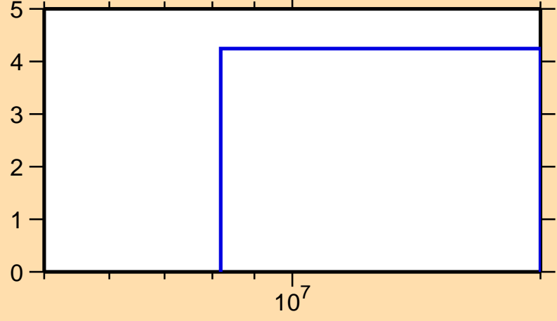
\Delta\sigma/\sigma vs. E for ^{94}\text{Zr}(n,\text{nonel.})
