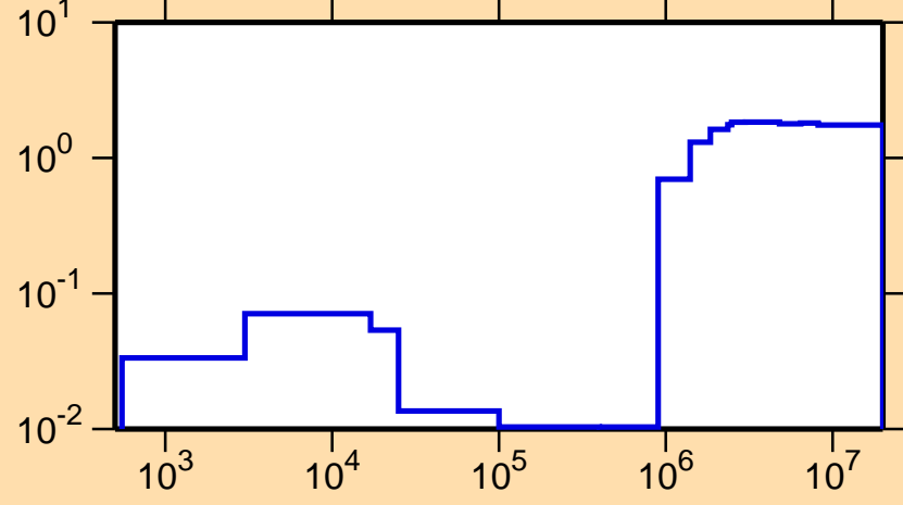
\sigma vs. E for ^{94}\text{Zr}(n,\text{nonel.})
