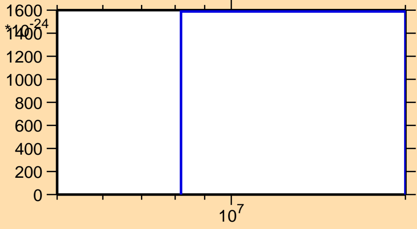
\sigma vs. E for ^{94}\text{Zr}(\text{mt } 34)
