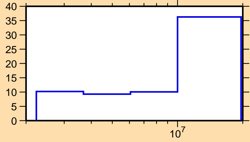
\Delta\sigma/\sigma vs. E for ^{95}\text{Zr}(n,\text{inel.})
