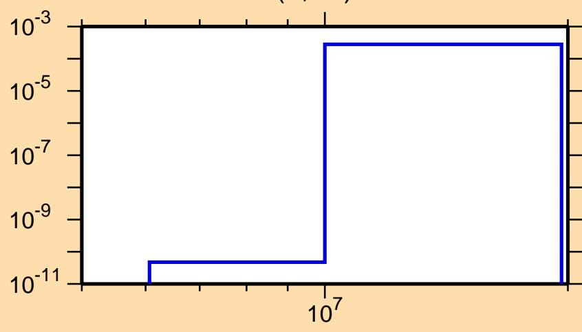
\sigma vs. E for ^{95}\text{Zr}(n,n\alpha)
