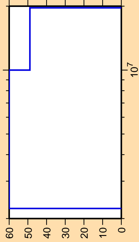
\Delta\sigma/\sigma vs. E for ^{95}\text{Zr}(n,\gamma)
