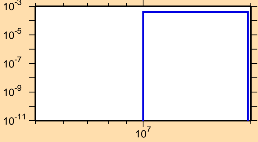
\sigma vs. E for ^{95}\text{Zr}(n,d)
