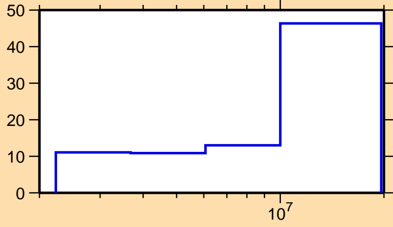
\Delta\sigma/\sigma vs. E for ^{95}\text{Zr}(n,n\text{cont.})
