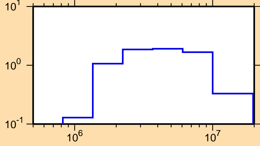
\sigma vs. E for ^{95}\text{Zr}(n,\text{inel.})
