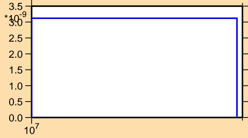
\sigma vs. E for ^{95}\text{Zr}(n,2n\alpha)
