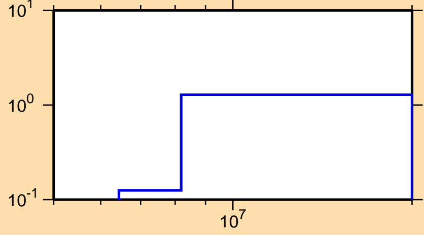
\sigma vs. E for ^{95}\text{Zr}(n,2n)
