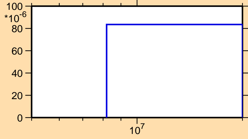
\sigma vs. E for ^{95}\text{Zr}(n,t)
