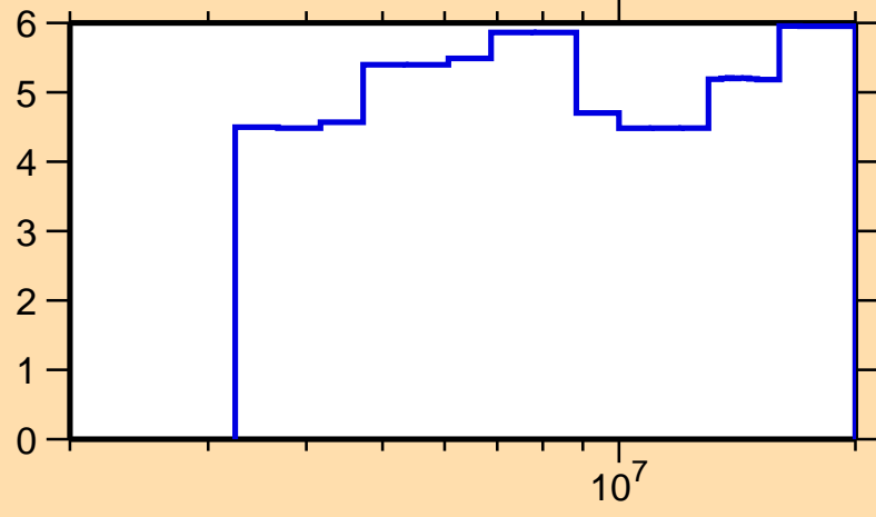
\Delta\sigma/\sigma vs. E for ^{96}\text{Zr}(n,nonel.)
