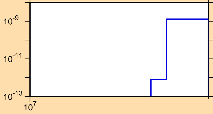
\sigma vs. E for ^{96}\text{Zr}(n,2n\alpha)
