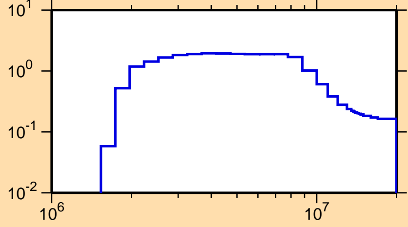
\sigma vs. E for ^{96}\text{Zr}(n,\text{inel.})
