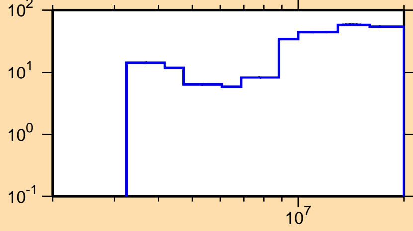
\Delta\sigma/\sigma vs. E for ^{96}\text{Zr}(n,n\text{cont.})
