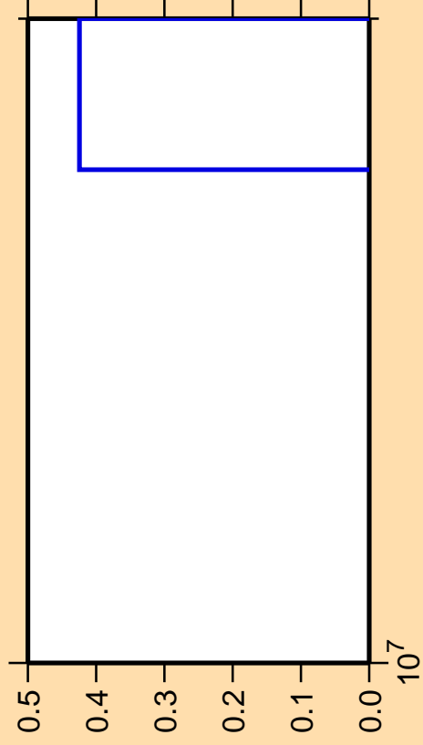
\Delta\sigma/\sigma vs. E for ^{96}\text{Zr}(n,2np)
