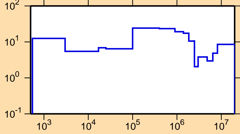
\Delta\sigma/\sigma vs. E for ^{96}\text{Zr}(n,\text{tot.})
