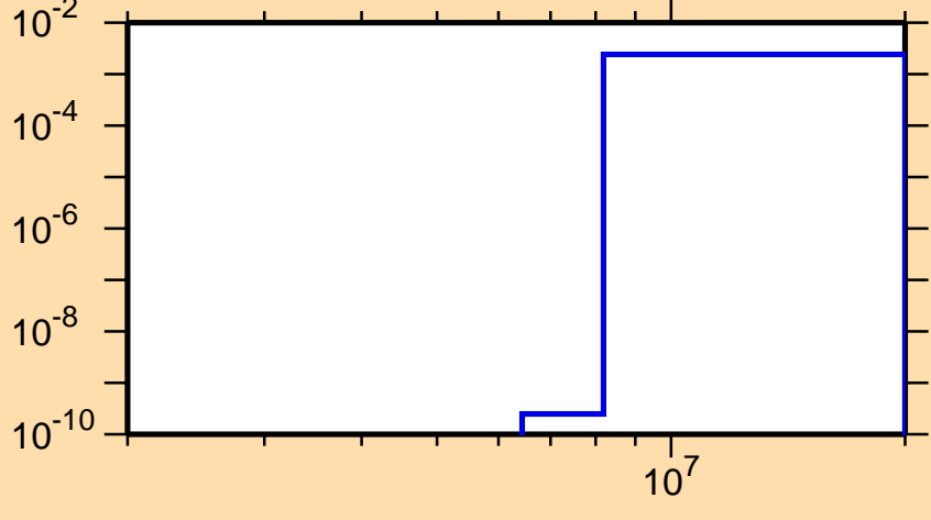
\sigma vs. E for ^{96}\text{Zr}(n,p)
