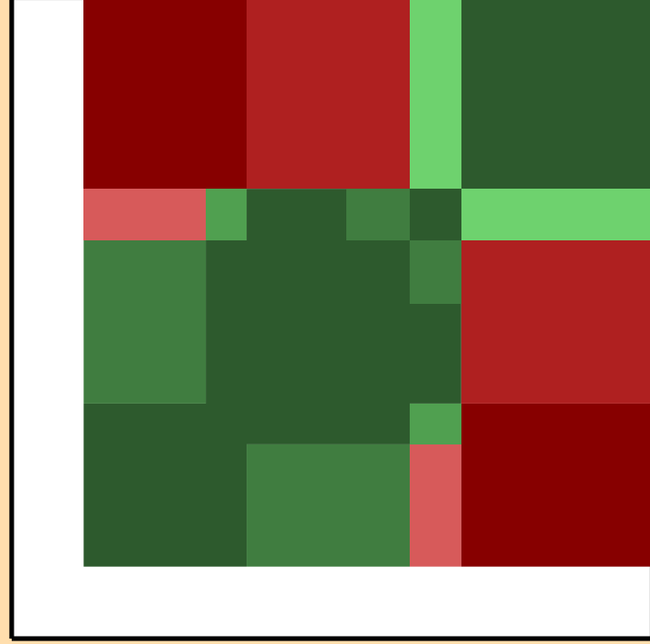
\sigma vs. E for ^{96}\text{Zr}(n,\text{inel.})
