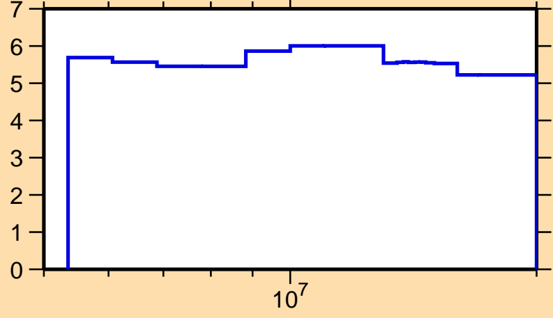
\Delta\sigma/\sigma vs. E for ^{97}\text{Zr}(n,\text{nonel.})
