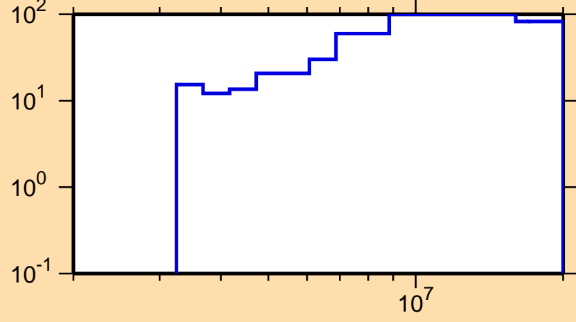
\Delta\sigma/\sigma vs. E for ^{97}\text{Zr}(n,n\text{cont.})
