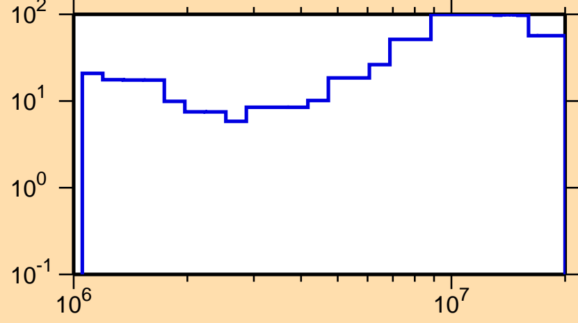
\Delta\sigma/\sigma vs. E for ^{97}\text{Zr}(n,\text{inel.})
