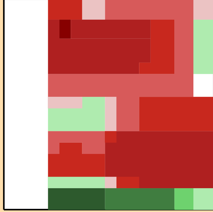
\Delta\sigma/\sigma vs. E for ^{97}\text{Zr}(n,n\text{cont.})
