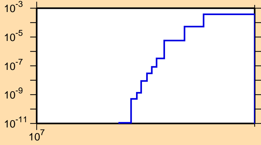
\sigma vs. E for ^{97}\text{Zr}(n,np)
