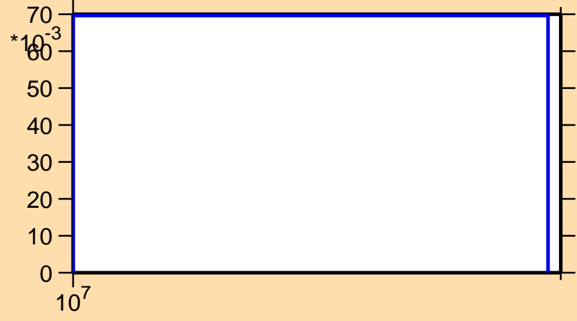
\sigma vs. E for ^{97}\text{Zr}(n,3n)
