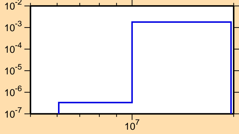
\sigma vs. E for ^{97}\text{Zr}(n,p)
