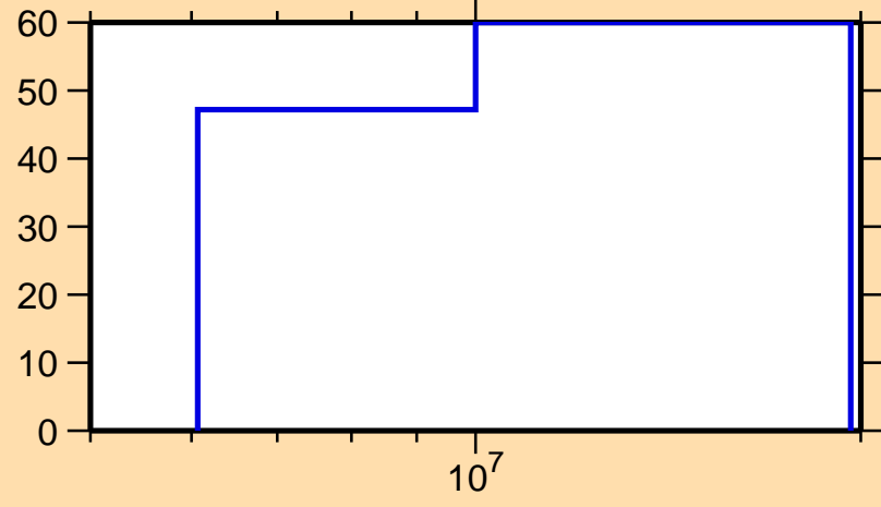
\Delta\sigma/\sigma vs. E for ^{97}\text{Zr}(n,ncont.)
