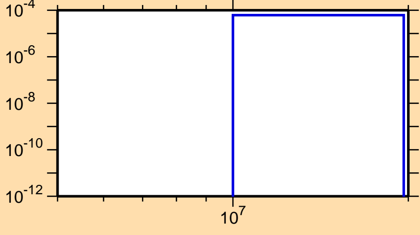
\sigma vs. E for ^{97}\text{Zr}(n,d)
