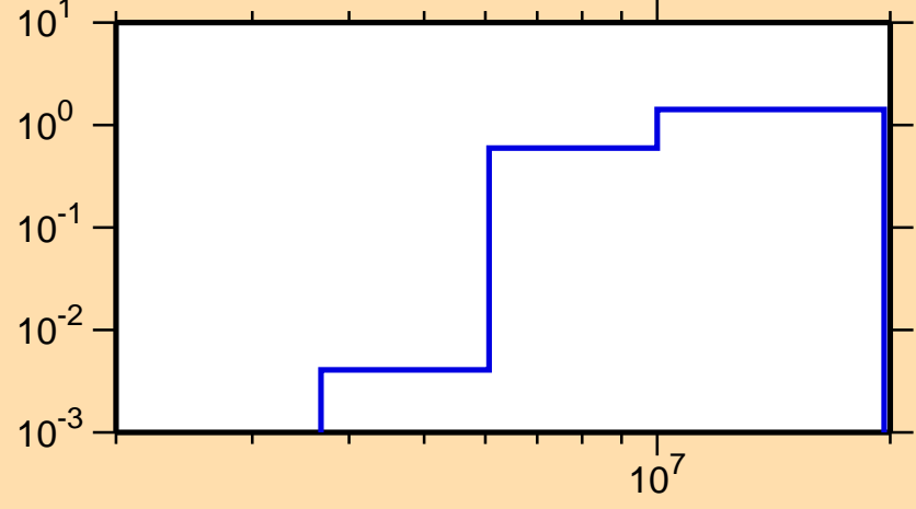
\sigma vs. E for ^{97}\text{Zr}(n,2n)
