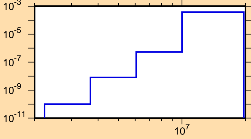
\sigma vs. E for ^{97}\text{Zr}(n,\alpha)
