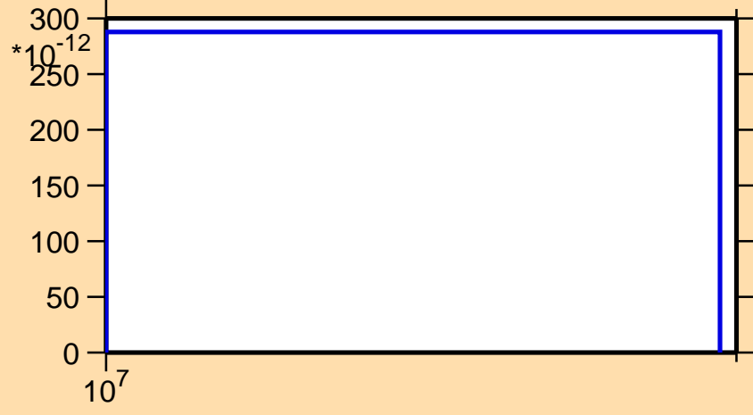
\sigma vs. E for ^{97}\text{Zr}(n,2n\alpha)
