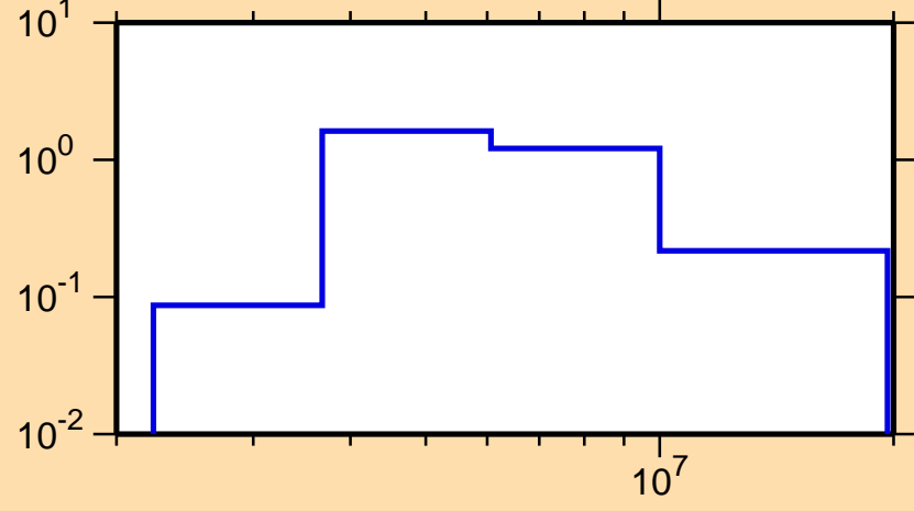
\sigma vs. E for ^{97}\text{Zr}(n,n\text{cont.})
