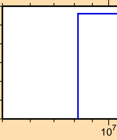
\sigma vs. E for ^{97}\text{Zr}(n,3n)
