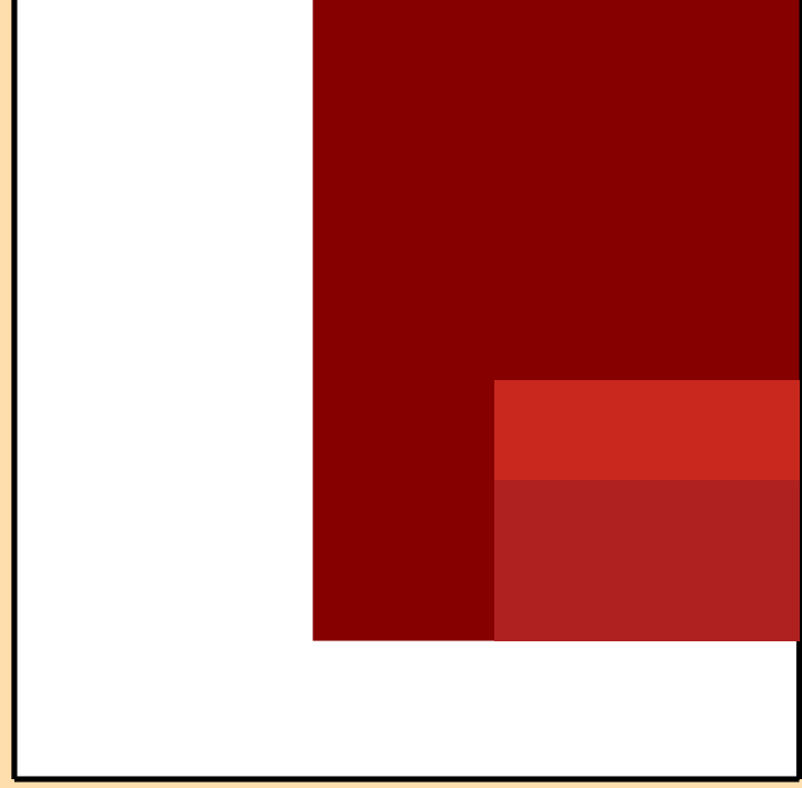
Correlation Matrix
