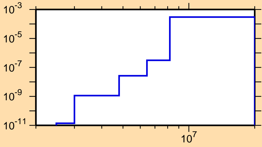
\sigma vs. E for ^{97}\text{Zr}(n,\alpha)
