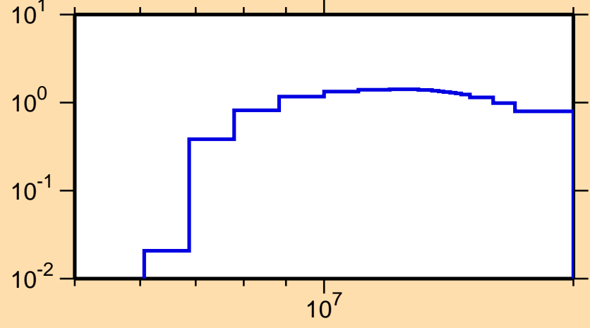
\sigma vs. E for ^{98}\text{Zr}(n,2n)
