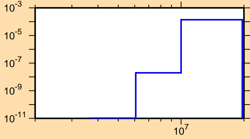
\sigma vs. E for ^{98}\text{Zr}(n,\alpha)
