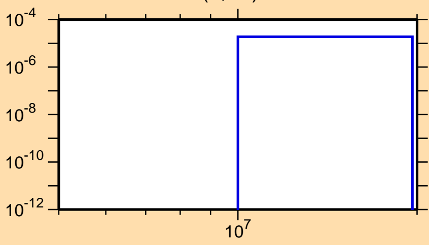
\sigma vs. E for ^{98}\text{Zr}(n,n\alpha)
