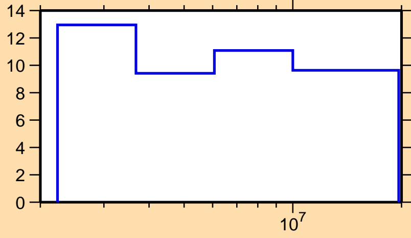
\Delta\sigma/\sigma vs. E for ^{98}\text{Zr}(n,nonel.)
