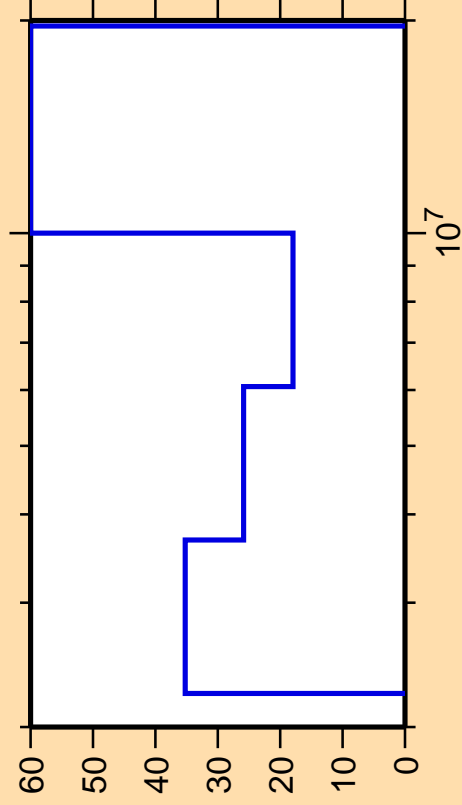
\Delta\sigma/\sigma vs. E for ^{98}\text{Zr}(n,ncont.)
