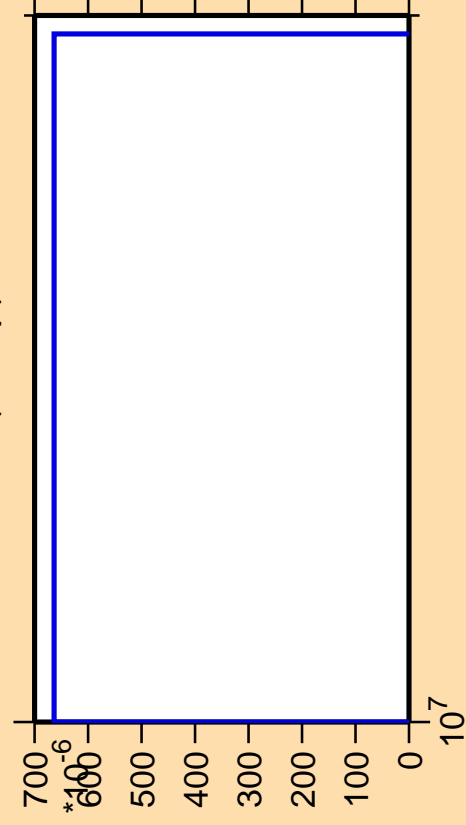
\Delta\sigma/\sigma vs. E for ^{98}\text{Zr}(n,2np)
