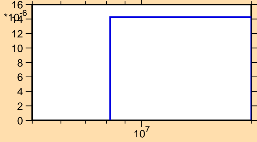
\sigma vs. E for ^{98}\text{Zr}(n,d)
