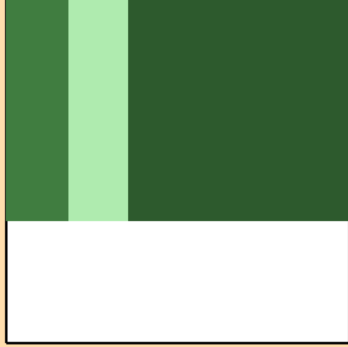
\Delta\sigma/\sigma vs. E for ^{98}\text{Zr}(n,\gamma)
