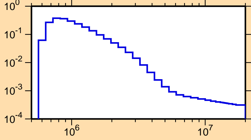
\sigma vs. E for ^{99}\text{Zr}(n,n_3)
