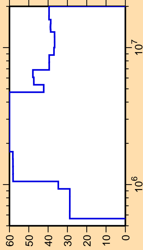
\Delta\sigma/\sigma vs. E for ^{99}\text{Zr}(n,n_3)
