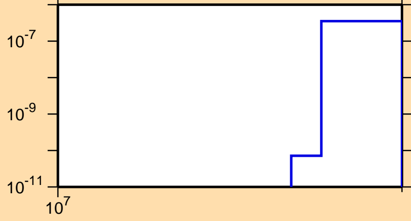
\sigma vs. E for ^{99}\text{Zr}(n,nt)
