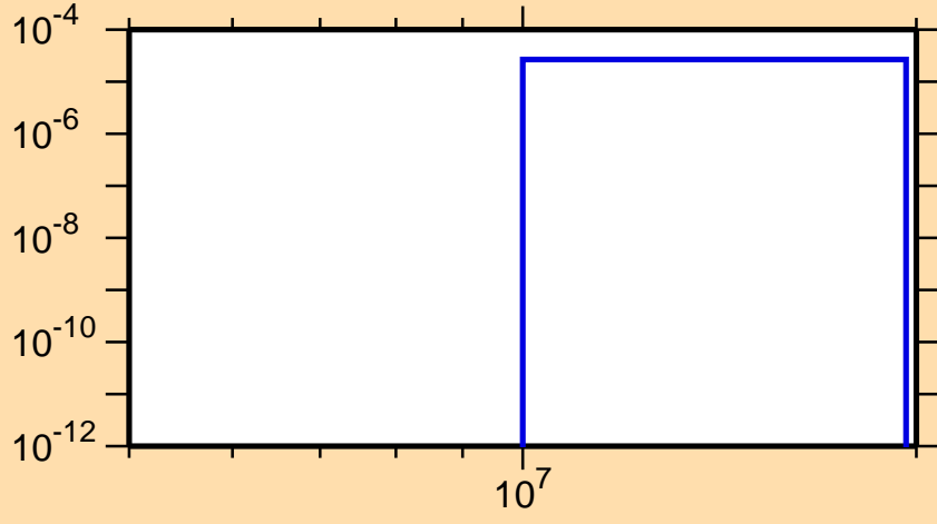
\sigma vs. E for ^{99}\text{Zr}(n,n\alpha)
