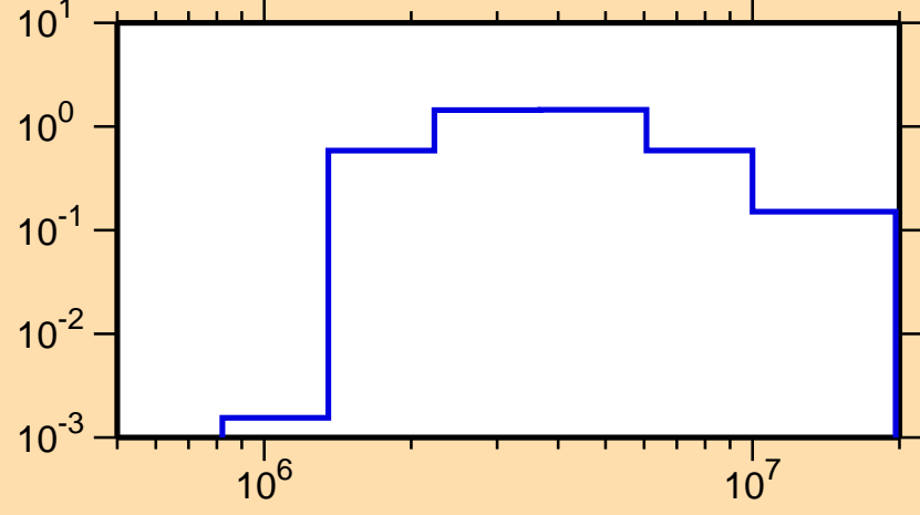
\sigma vs. E for ^{99}\text{Zr}(n,n\text{cont.})
