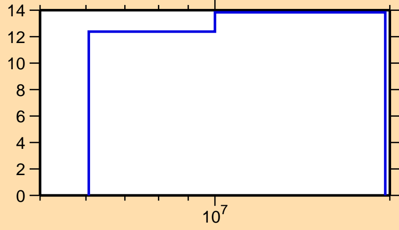
\Delta\sigma/\sigma vs. E for ^{99}\text{Zr}(n,el.)
