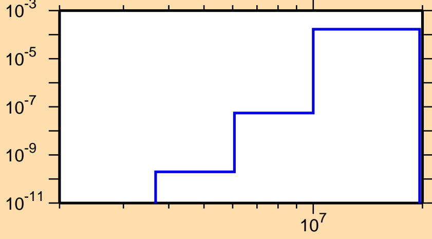
\sigma vs. E for ^{99}\text{Zr}(n,\alpha)
