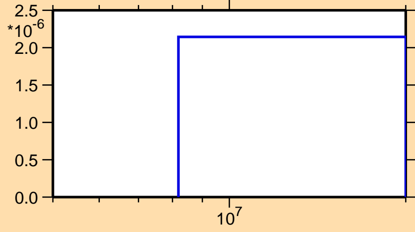
\sigma vs. E for ^{99}\text{Zr}(n,np)
