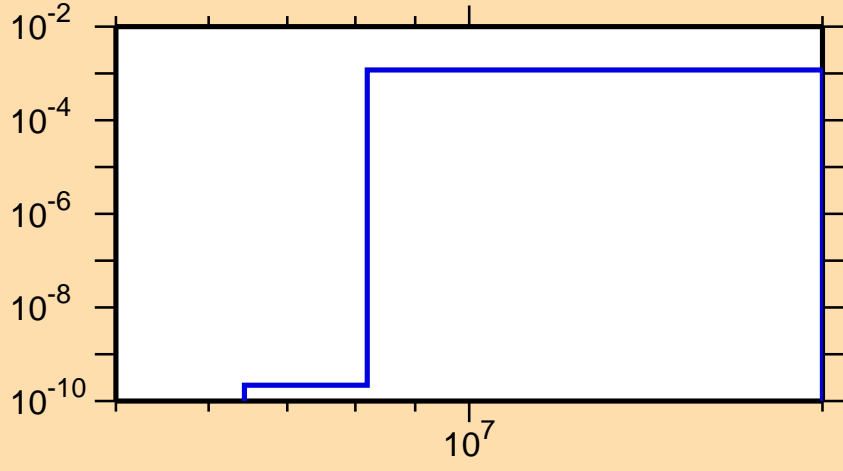
\sigma vs. E for ^{99}\text{Zr}(n,p)
