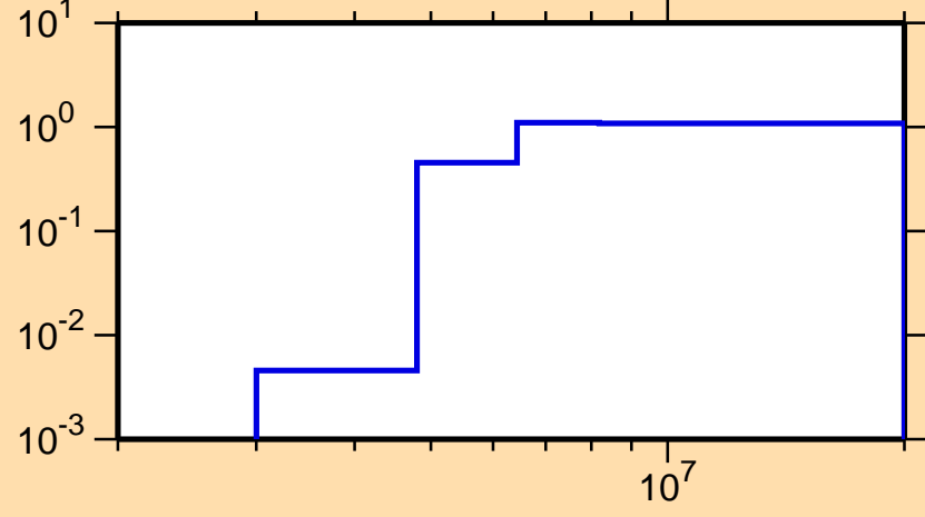
\sigma vs. E for ^{99}\text{Zr}(n,2n)
