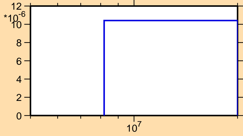
\sigma vs. E for ^{99}\text{Zr}(n,t)
