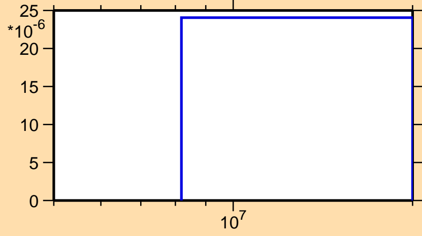
\sigma vs. E for ^{99}\text{Zr}(n,d)
