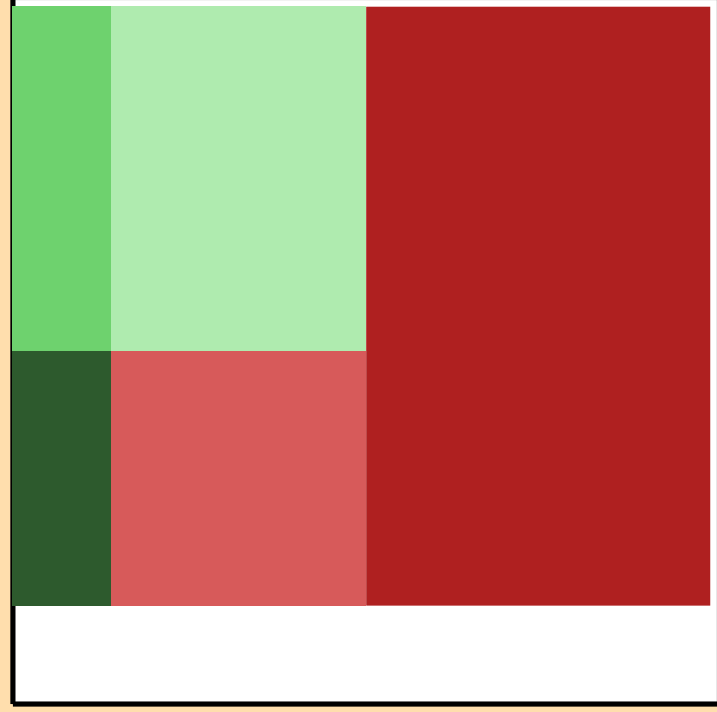
\Delta\sigma/\sigma vs. E for ^{100}\text{Zr}(n,\text{inel.})
