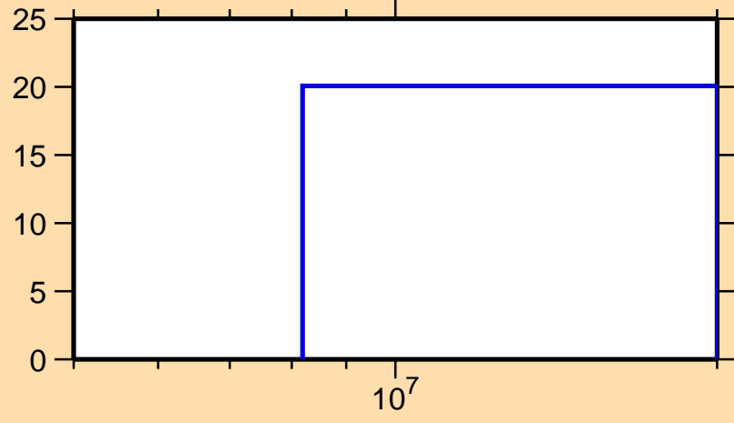
\Delta\sigma/\sigma vs. E for ^{100}\text{Zr}(n,el.)
