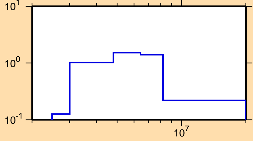
\sigma vs. E for ^{100}\text{Zr}(n,n\text{cont.})
