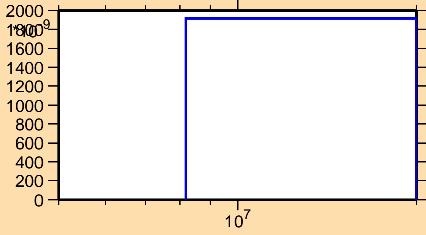
\sigma vs. E for ^{100}\text{Zr}(n,n\alpha)
