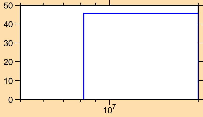
\Delta\sigma/\sigma vs. E for ^{100}\text{Zr}(n,ncont.)
