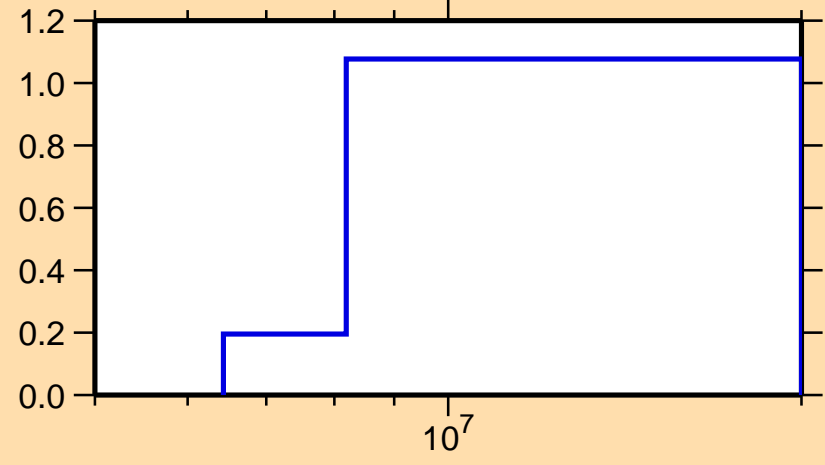
\sigma vs. E for ^{100}\text{Zr}(n,2n)
