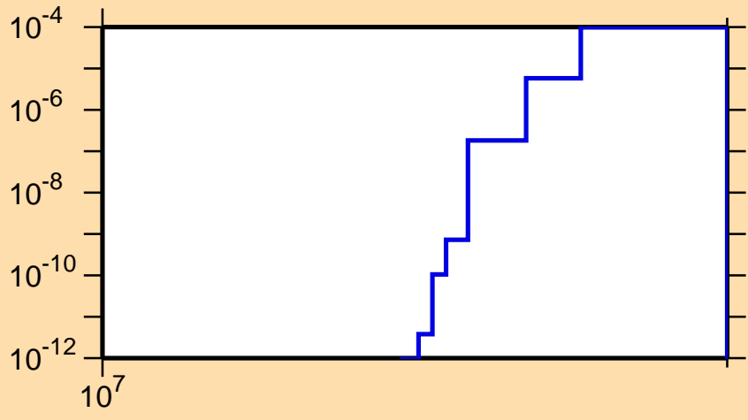
\sigma vs. E for ^{101}\text{Zr}(n,np)
