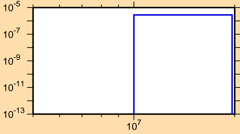
\sigma vs. E for ^{101}\text{Zr}(n,t)
