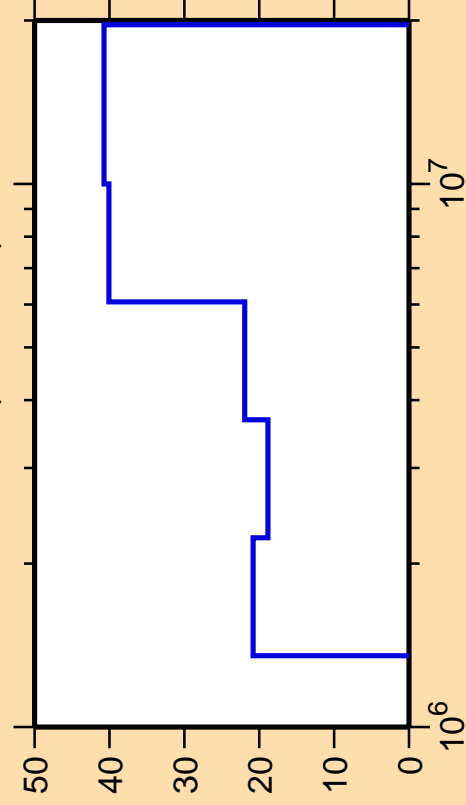
\Delta\sigma/\sigma vs. E for ^{101}\text{Zr}(n,n\text{cont.})
