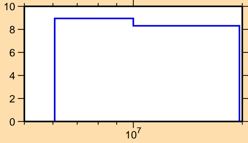
\Delta\sigma/\sigma vs. E for ^{101}\text{Zr}(n,el.)
