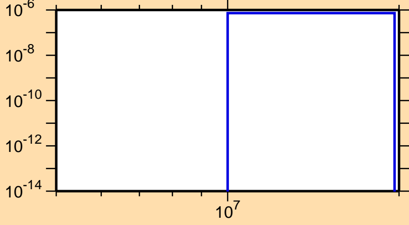
\sigma vs. E for ^{101}\text{Zr}(n,n\alpha)
