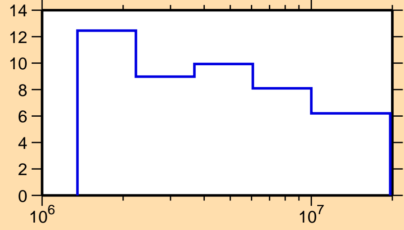
\Delta\sigma/\sigma vs. E for ^{101}\text{Zr}(n,n\text{onel.})
