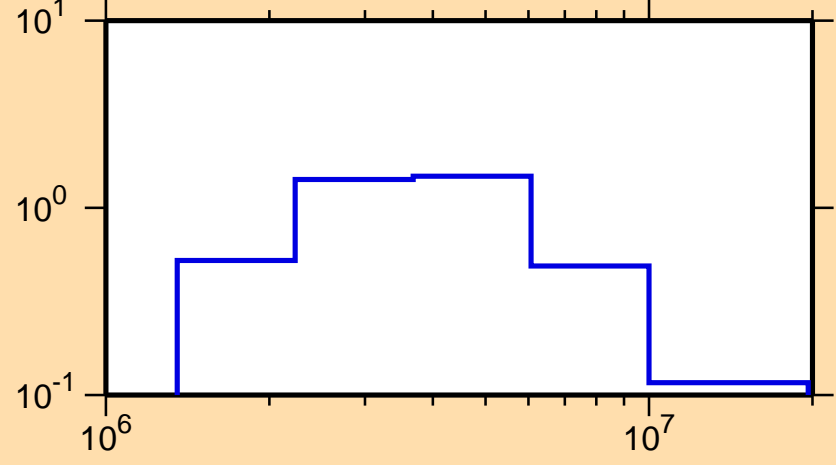
\sigma vs. E for ^{101}\text{Zr}(n,n\text{cont.})
