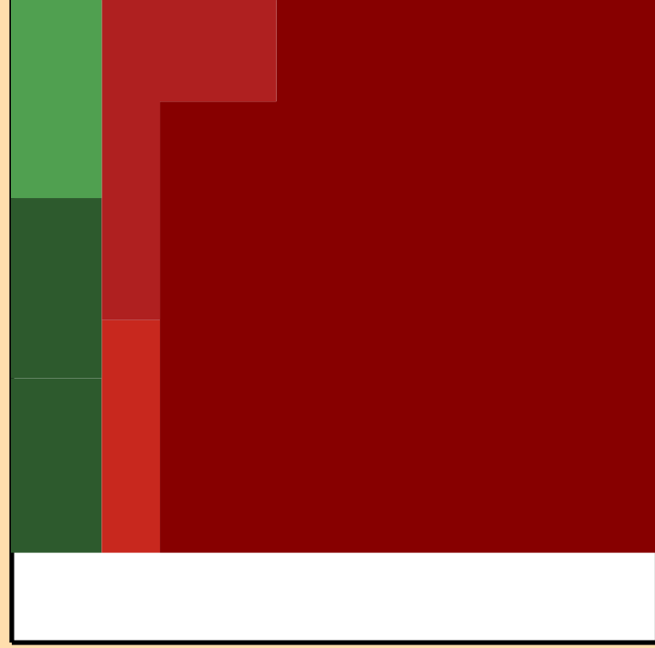
\Delta\sigma/\sigma vs. E for ^{102}\text{Zr}(n,\text{inel.})
