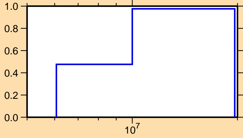
\sigma vs. E for ^{102}\text{Zr}(n,2n)
