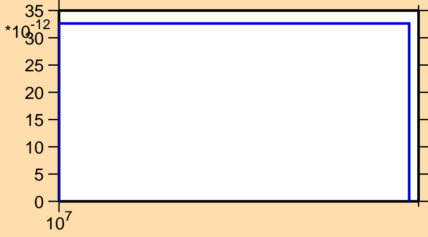
\sigma vs. E for ^{102}\text{Zr}(n,nt)
