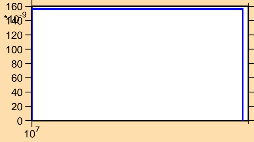
\sigma vs. E for ^{102}\text{Zr}(n,n\alpha)
