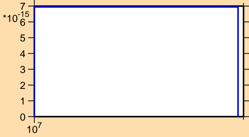
\sigma vs. E for ^{102}\text{Zr}(n,2n\alpha)
