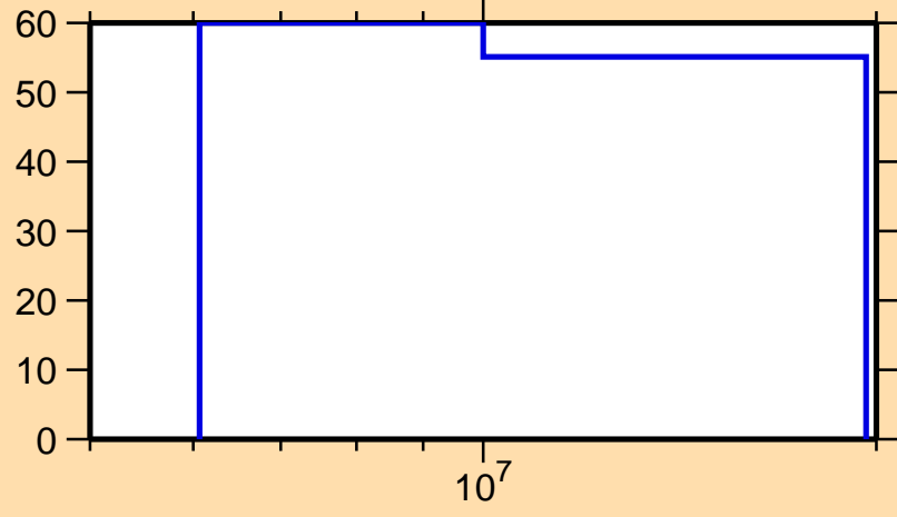
\Delta\sigma/\sigma vs. E for ^{102}\text{Zr}(n,2n)
