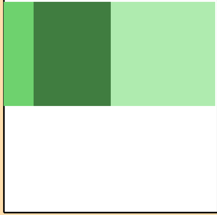
\Delta\sigma/\sigma vs. E for ^{102}\text{Zr}(n,n_1)
