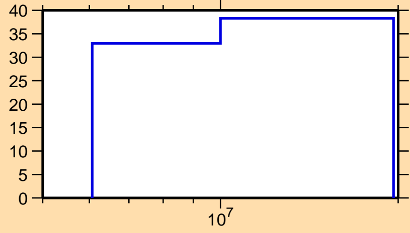
\Delta\sigma/\sigma vs. E for ^{102}\text{Zr}(n,\text{nonel.})
