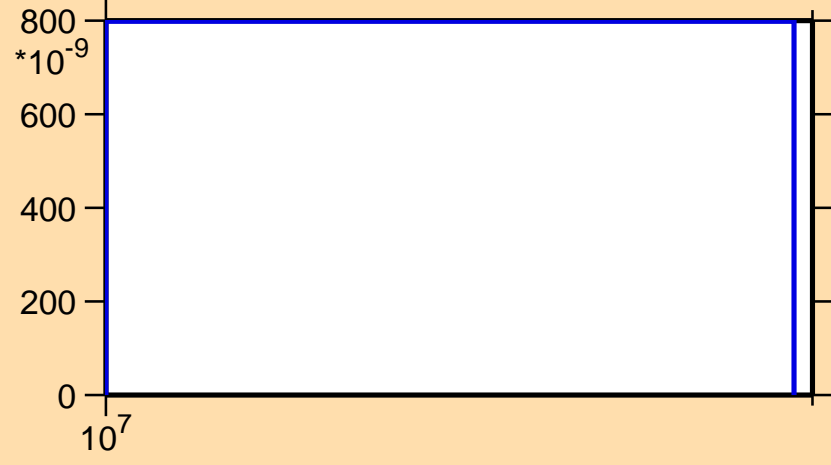
\sigma vs. E for ^{102}\text{Zr}(n,t)
