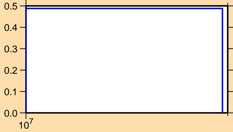
\sigma vs. E for ^{102}\text{Zr}(n,3n)
