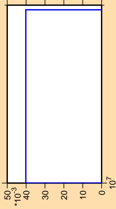
\Delta\sigma/\sigma vs. E for ^{102}\text{Zr}(n,2n\alpha)
