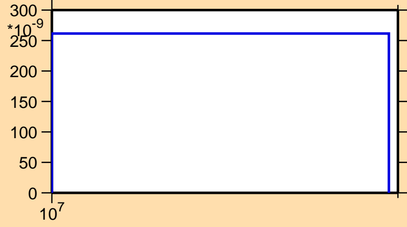
\sigma vs. E for ^{102}\text{Zr}(n,np)
