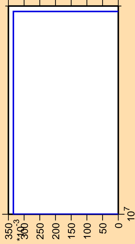
\Delta\sigma/\sigma vs. E for ^{102}\text{Zr}(n,\text{nd})
