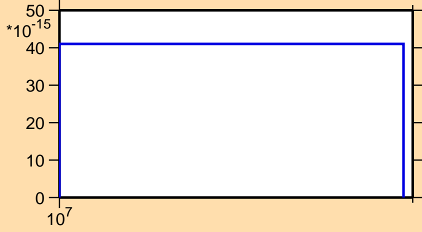
\sigma vs. E for ^{102}\text{Zr}(n,\text{nd})
