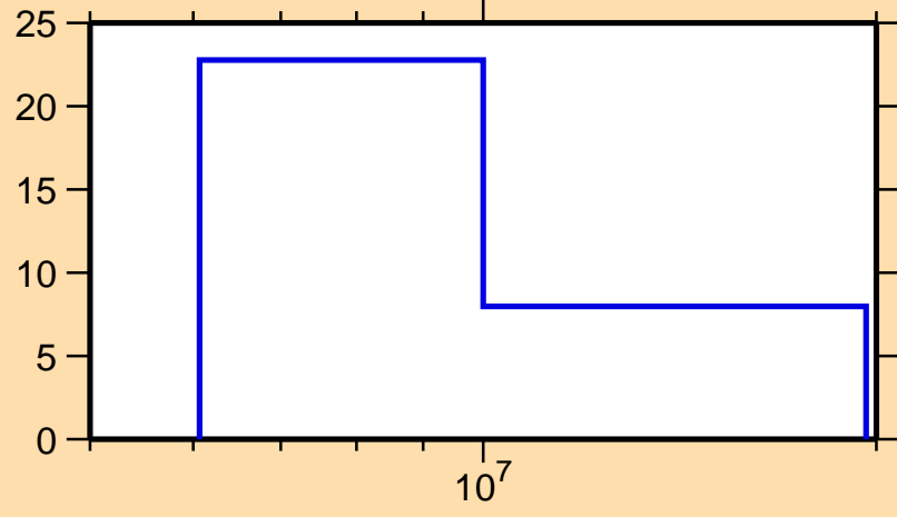
\Delta\sigma/\sigma vs. E for ^{102}\text{Zr}(n,el.)
