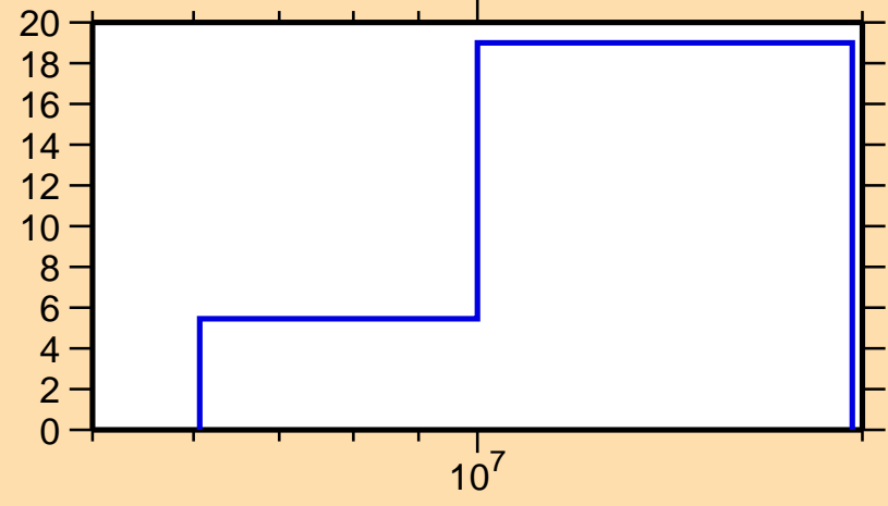
\Delta\sigma/\sigma vs. E for ^{102}\text{Zr}(n,\text{tot.})
