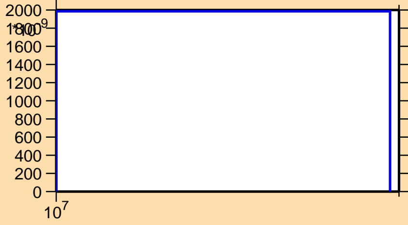
\sigma vs. E for ^{102}\text{Zr}(n,d)
