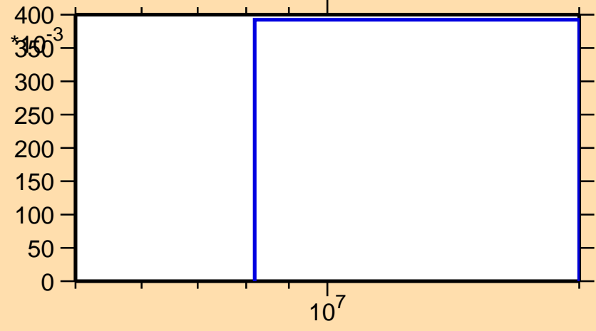
\sigma vs. E for ^{102}\text{Zr}(n,3n)
