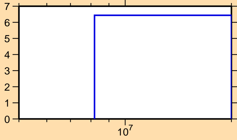
\Delta\sigma/\sigma vs. E for ^{102}\text{Zr}(n,\text{el.})
