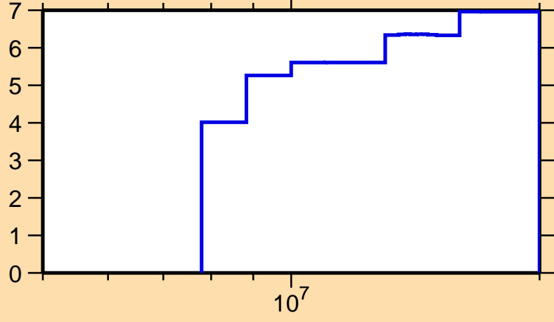
\Delta\sigma/\sigma vs. E for ^{103}\text{Zr}(n,tot.)
