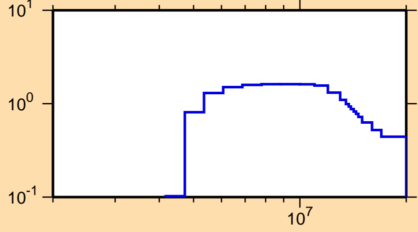
\sigma vs. E for ^{103}\text{Zr}(n,2n)
