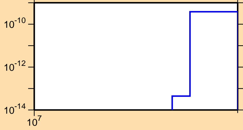
\sigma vs. E for ^{103}\text{Zr}(n,2n\alpha)
