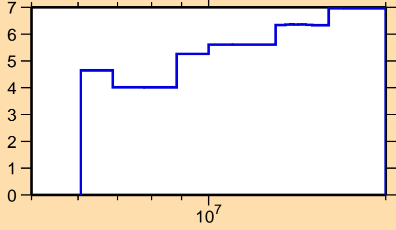
\Delta\sigma/\sigma vs. E for ^{103}\text{Zr}(n,\text{tot.})
