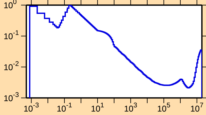
\sigma vs. E for ^{214}\text{Ac}(n,\alpha)
