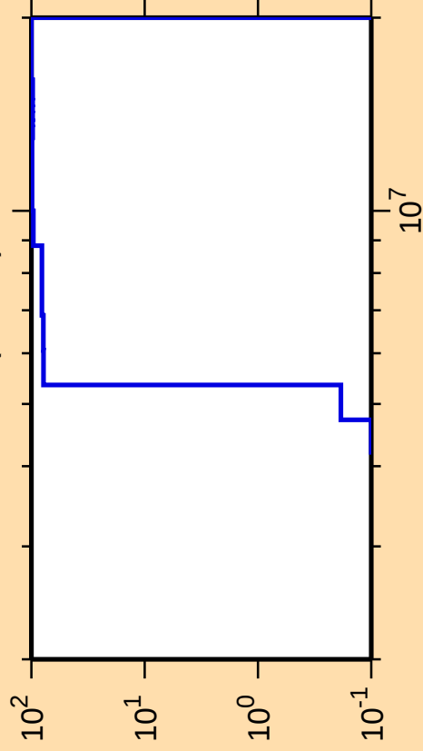
\Delta\sigma/\sigma vs. E for ^{214}\text{Ac}(\text{mt } 45)
