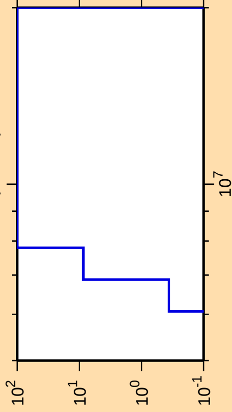
\Delta\sigma/\sigma vs. E for ^{214}\text{Ac}(n,\text{He3})
