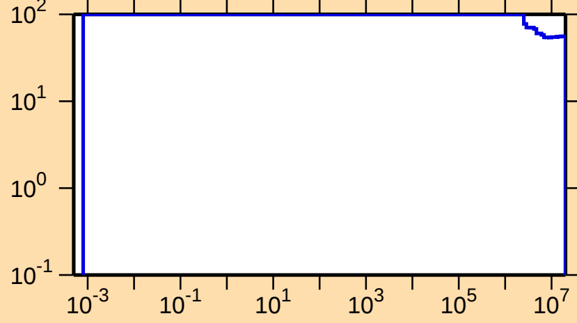
\Delta\sigma/\sigma vs. E for ^{214}\text{Ac}(n,p)
