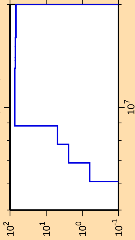
\Delta\sigma/\sigma vs. E for ^{214}\text{Ac}(n,2n\alpha)
