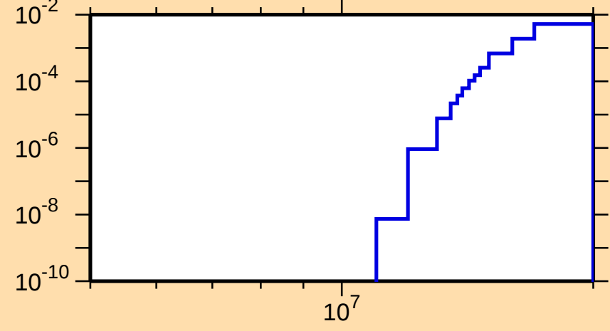
\sigma vs. E for ^{214}\text{Ac}(n,2np)
