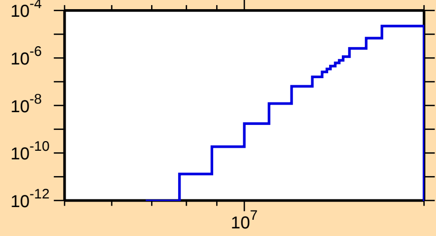
\sigma vs. E for ^{214}\text{Ac}(n,\text{He3})
