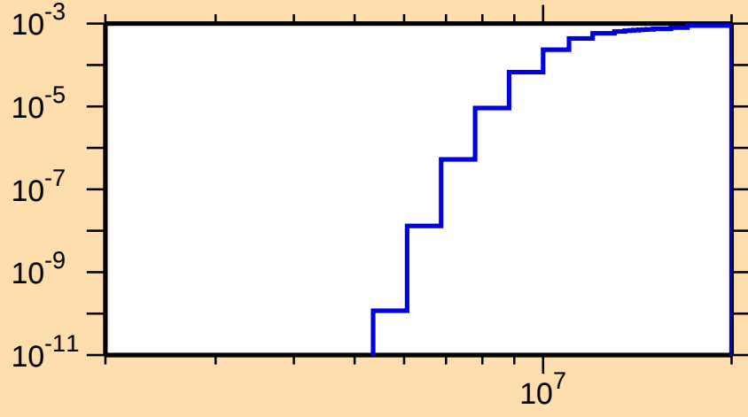
\sigma vs. E for ^{214}\text{Ac}(\text{mt } 45)
