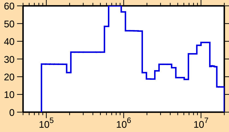
\Delta\sigma/\sigma vs. E for ^{214}\text{Ac}(n,\text{el.})
