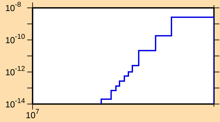
\sigma vs. E for ^{214}\text{Ac}(\text{mt } 34)
