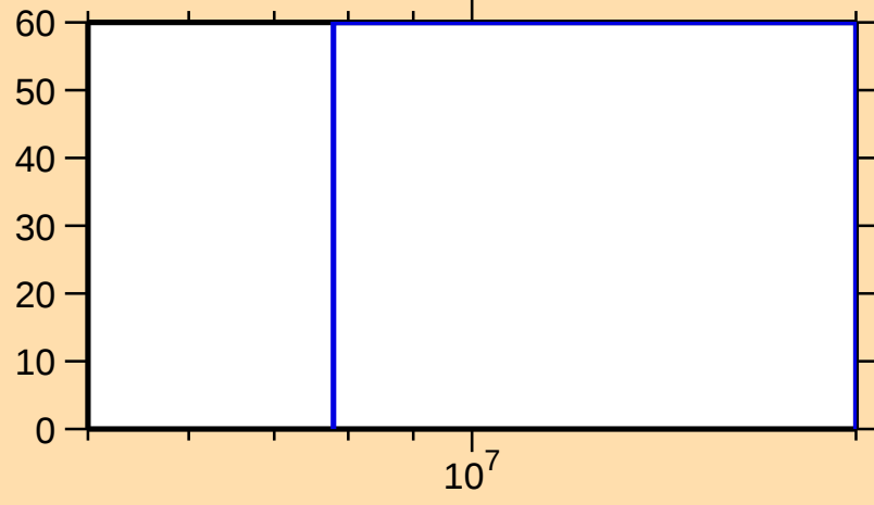
\Delta\sigma/\sigma vs. E for ^{214}\text{Ac}(n,2n)
