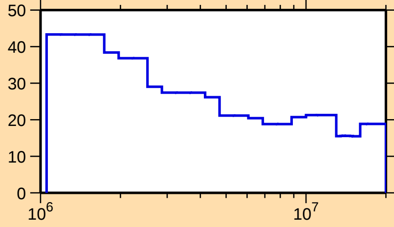
\Delta\sigma/\sigma vs. E for ^{214}\text{Ac}(n,n\text{onel.})
