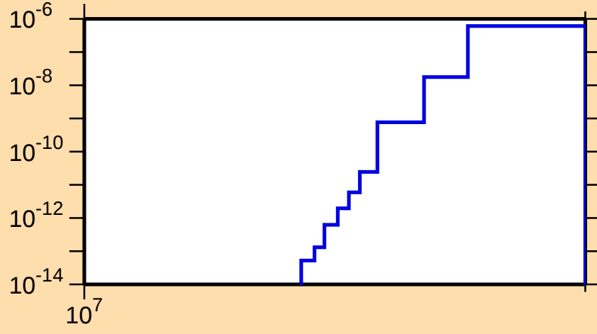
\sigma vs. E for ^{214}\text{Ac}(n,nt)
