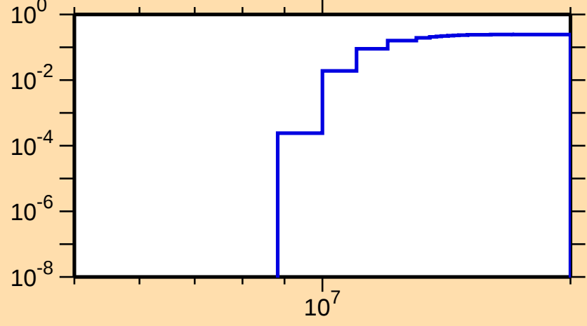
\sigma vs. E for ^{214}\text{Ac}(n,2n\alpha)
