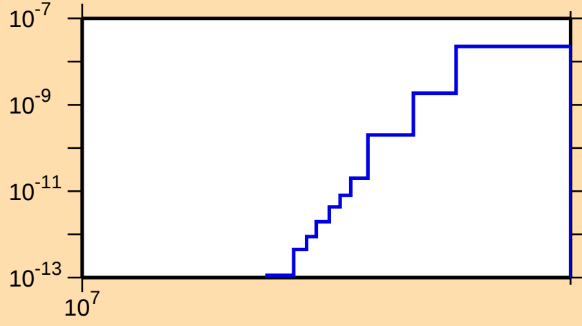
\sigma vs. E for ^{214}\text{Ac}(n,\text{pt})
