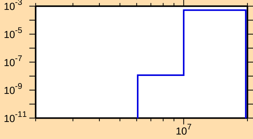
\sigma vs. E for ^{214}\text{Ac}(n,t)
