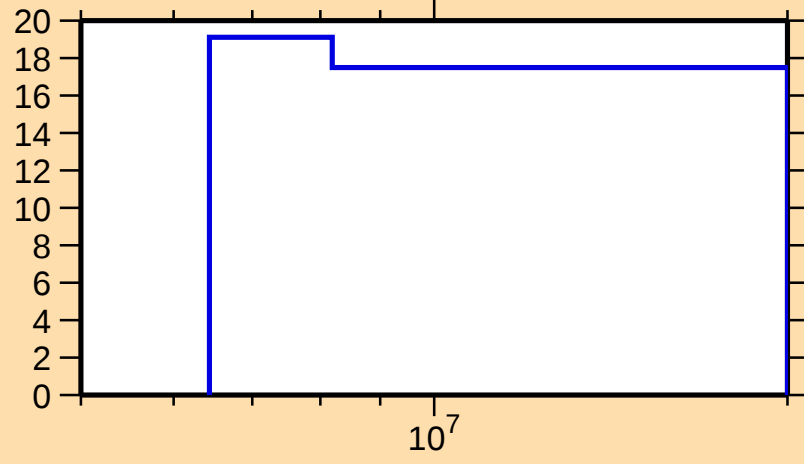
\Delta\sigma/\sigma vs. E for ^{214}\text{Ac}(n,\text{nonel.})
