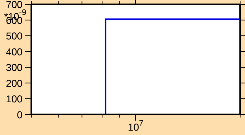
\sigma vs. E for ^{214}\text{Ac}(n,3n\alpha)
