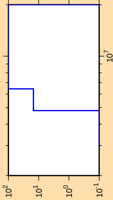
\Delta\sigma/\sigma vs. E for ^{214}\text{Ac}(n,t)
