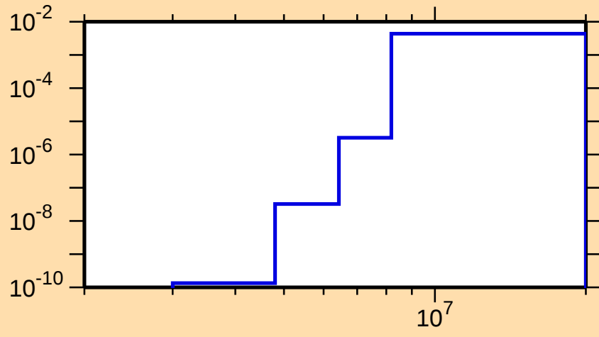
\sigma vs. E for ^{214}\text{Ac}(n,d)
