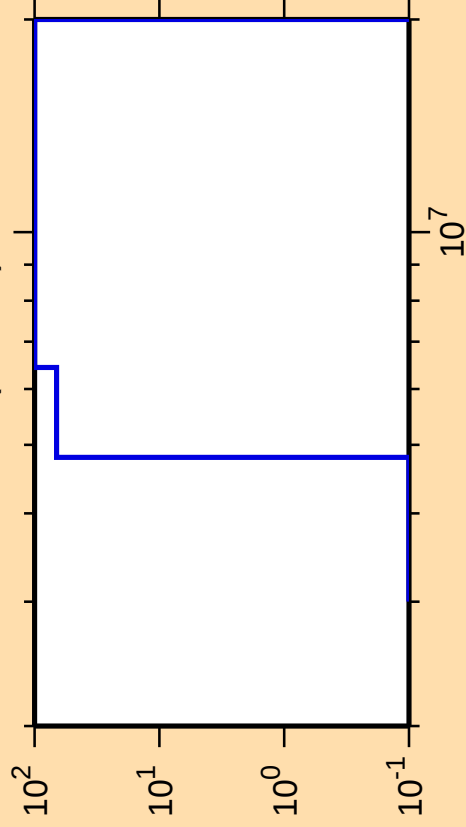
\Delta\sigma/\sigma vs. E for ^{214}\text{Ac}(\text{mt117})
