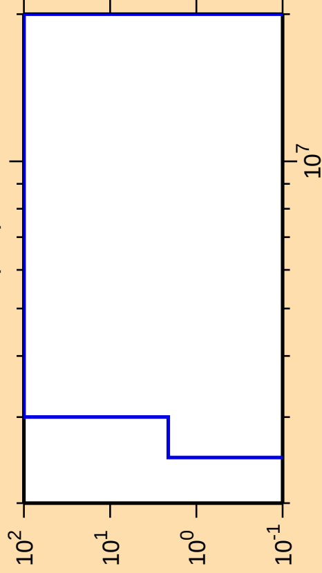
\Delta\sigma/\sigma vs. E for ^{214}\text{Ac}(n,d)
