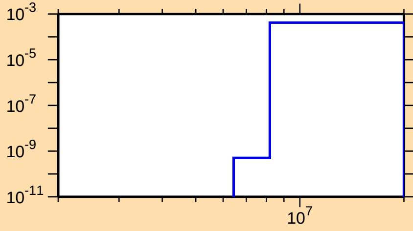
\sigma vs. E for ^{214}\text{Ac}(n,t)
