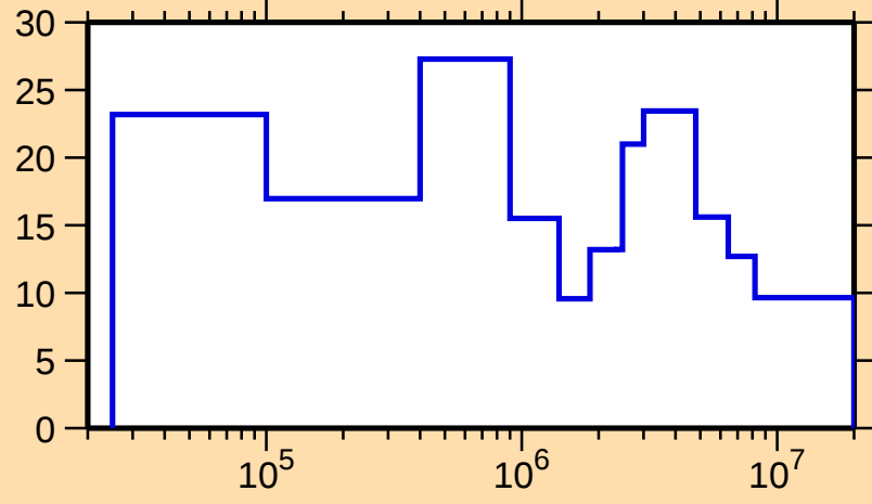
\Delta\sigma/\sigma vs. E for ^{214}\text{Ac}(n,\text{tot.})
