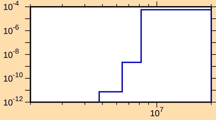
\sigma vs. E for ^{214}\text{Ac}(\text{mt117})
