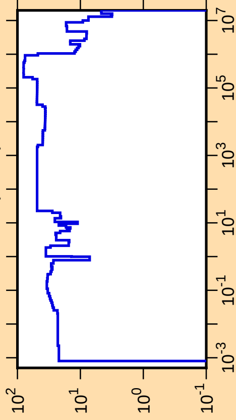
\Delta\sigma/\sigma vs. E for ^{222}\text{Ac}(n,\text{tot.})
