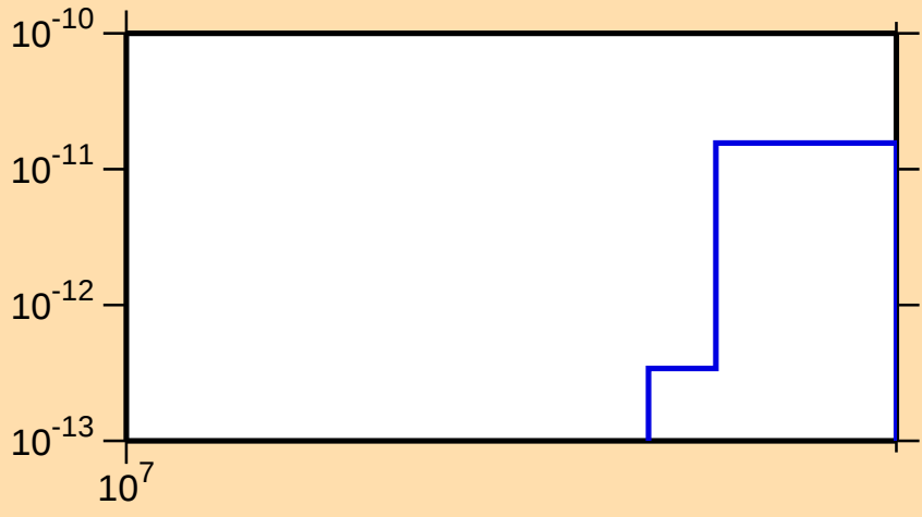
\sigma vs. E for ^{222}\text{Ac}(\text{mt } 34)
