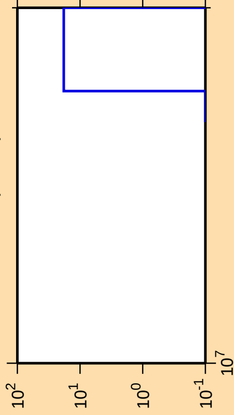
\Delta\sigma/\sigma vs. E for ^{222}\text{Ac}(\text{mt } 42)
