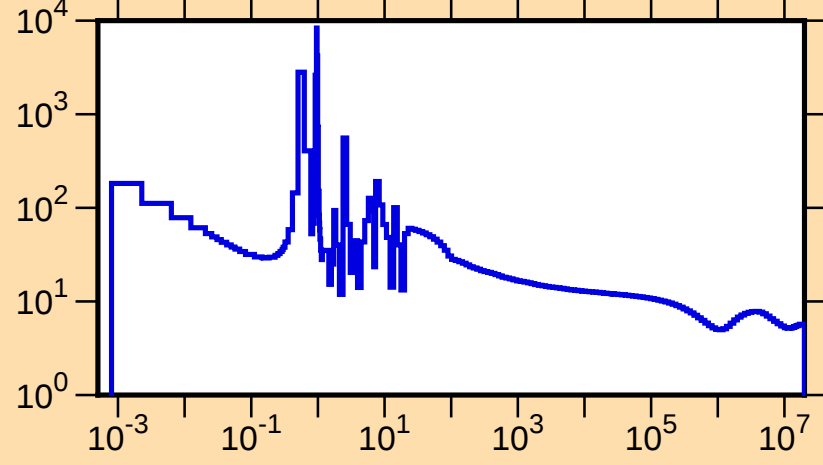
\sigma vs. E for ^{222}\text{Ac}(n,\text{tot.})
