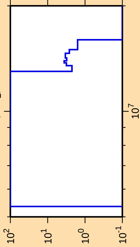
\Delta\sigma/\sigma vs. E for ^{222}\text{Ac}(n,n_1)
