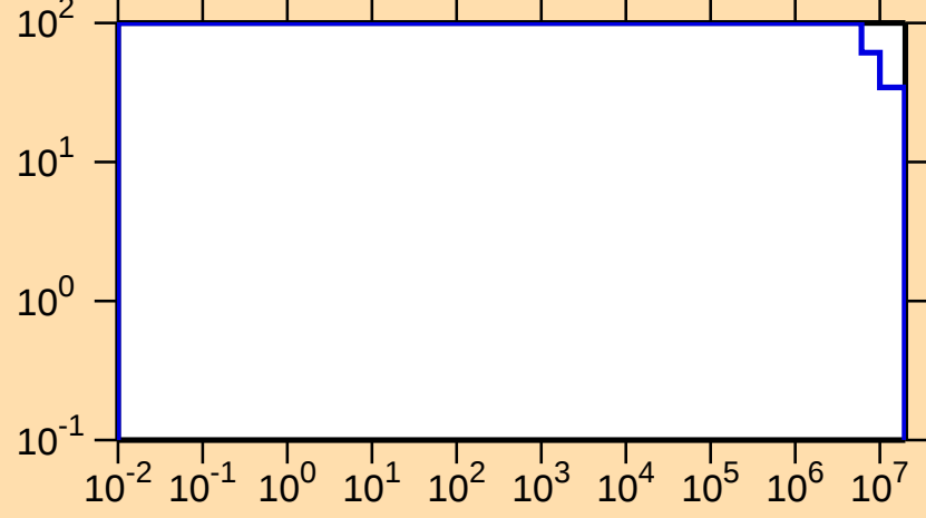
\Delta\sigma/\sigma vs. E for ^{222}\text{Ac}(n,p)
