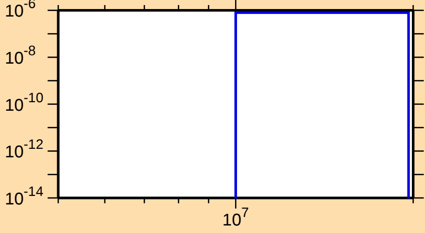
\sigma vs. E for ^{222}\text{Ac}(n,\text{nt})
