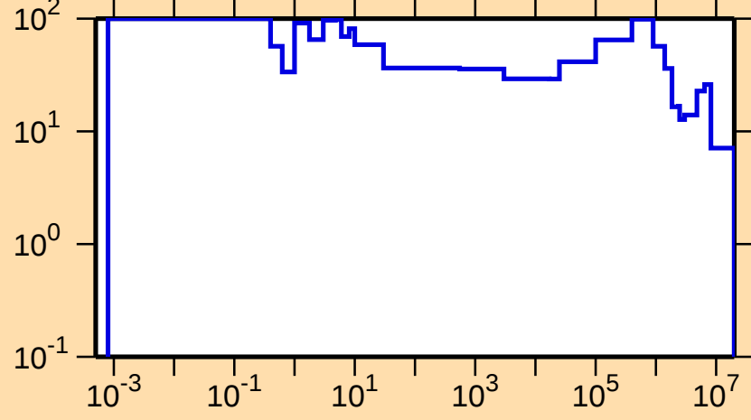
\Delta\sigma/\sigma vs. E for ^{222}\text{Ac}(n,\text{el.})
