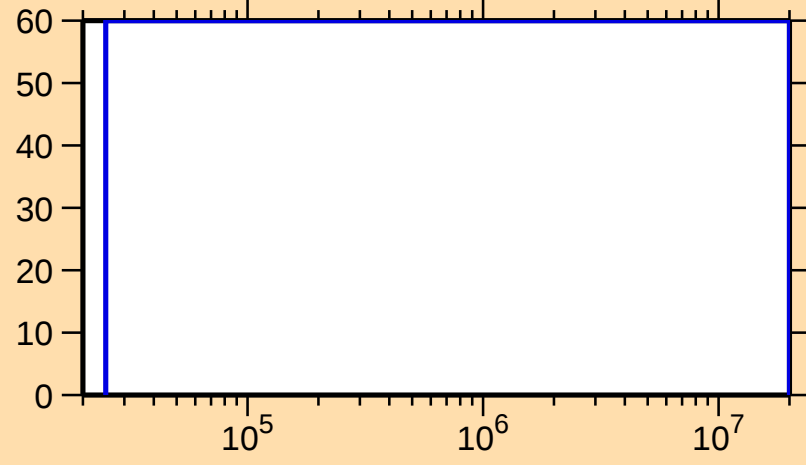
\Delta\sigma/\sigma vs. E for ^{222}\text{Ac}(n,n_1)
