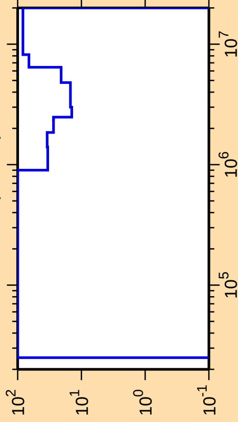
\Delta\sigma/\sigma vs. E for ^{222}\text{Ac}(n,\text{inel.})
