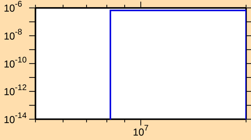
\sigma vs. E for ^{222}\text{Ac}(n,nt)
