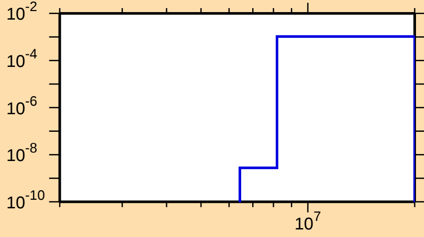
\sigma vs. E for ^{222}\text{Ac}(n,d)
