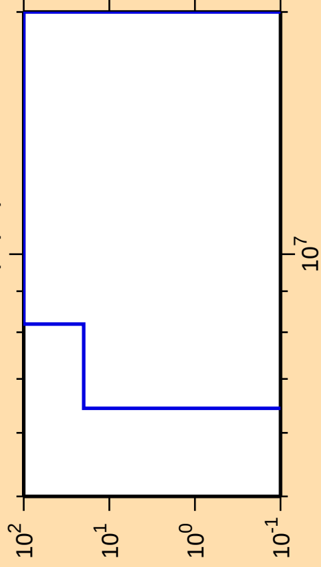
\Delta\sigma/\sigma vs. E for ^{222}\text{Ac}(n,p\alpha)
