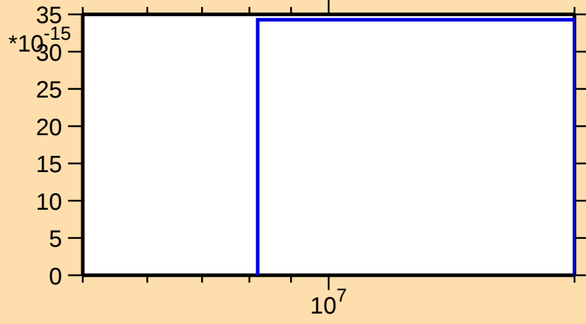
\sigma vs. E for ^{222}\text{Ac}(\text{mt } 42)
