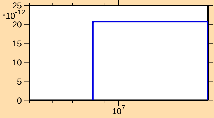
\sigma vs. E for ^{222}\text{Ac}(\text{mt } 45)
