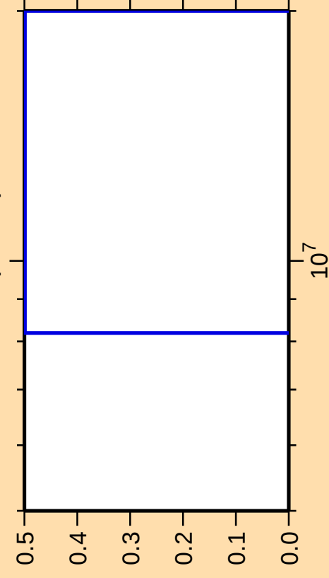
\Delta\sigma/\sigma vs. E for ^{222}\text{Ac}(\text{mt 11})
