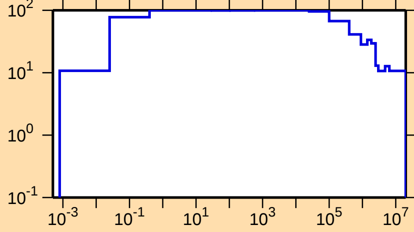
\Delta\sigma/\sigma vs. E for ^{222}\text{Ac}(n,\text{nonel.})
