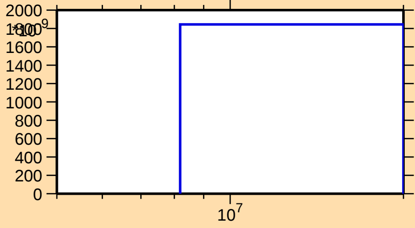
\sigma vs. E for ^{222}\text{Ac}(n,2np)
