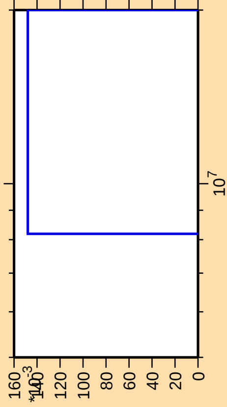
\Delta\sigma/\sigma vs. E for ^{222}\text{Ac}(\text{mt } 42)
