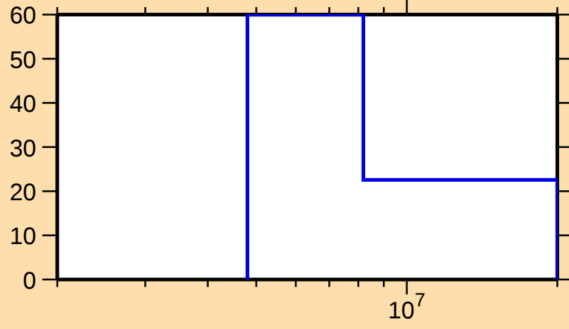
\Delta\sigma/\sigma vs. E for ^{222}\text{Ac}(n,2n)
