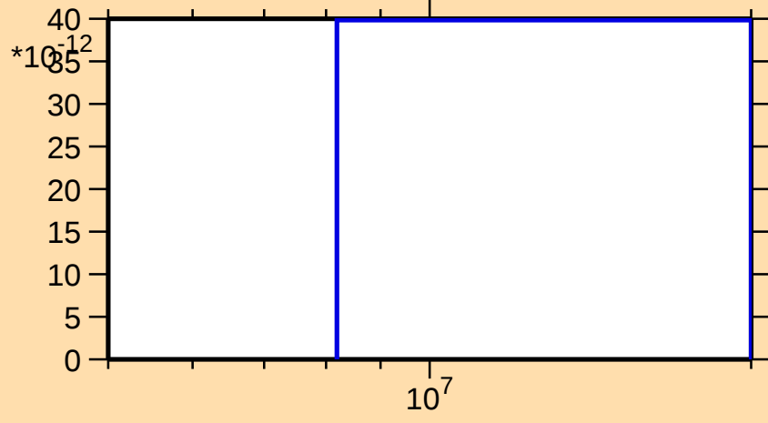
\sigma vs. E for ^{222}\text{Ac}(\text{mt117})
