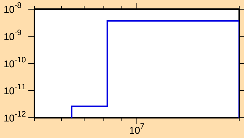
\sigma vs. E for ^{222}\text{Ac}(n,p\alpha)
