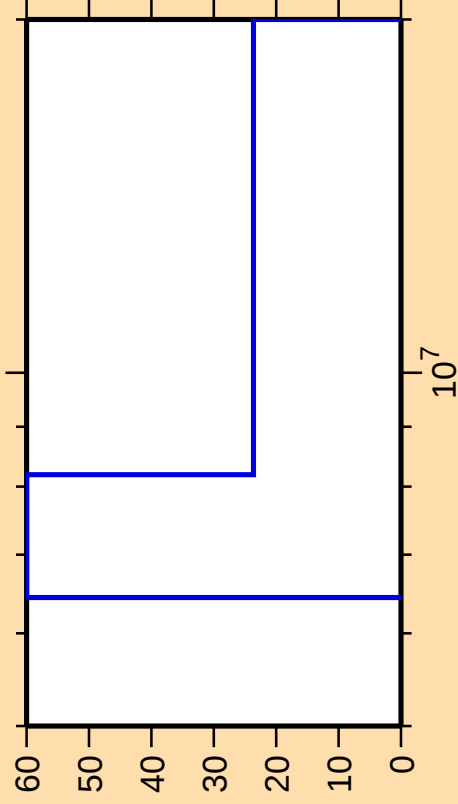
\Delta\sigma/\sigma vs. E for ^{222}\text{Ac}(n,2n\alpha)
