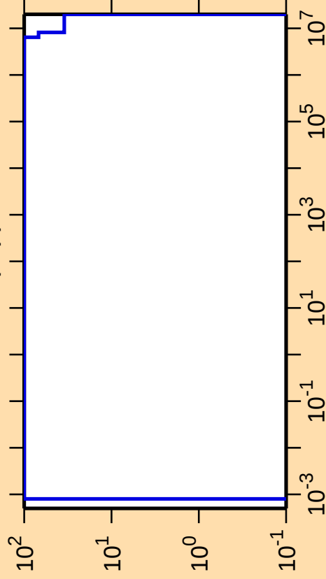
\Delta\sigma/\sigma vs. E for ^{222}\text{Ac}(n,p)
