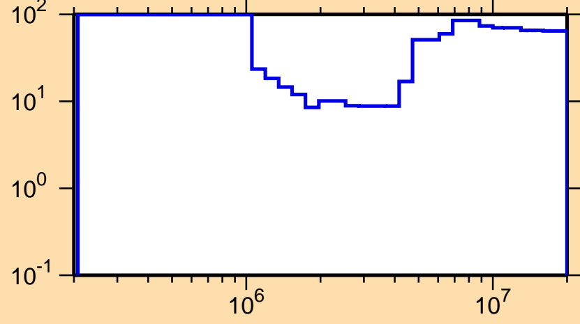
\Delta\sigma/\sigma vs. E for ^{222}\text{Ac}(n,n\text{cont.})
