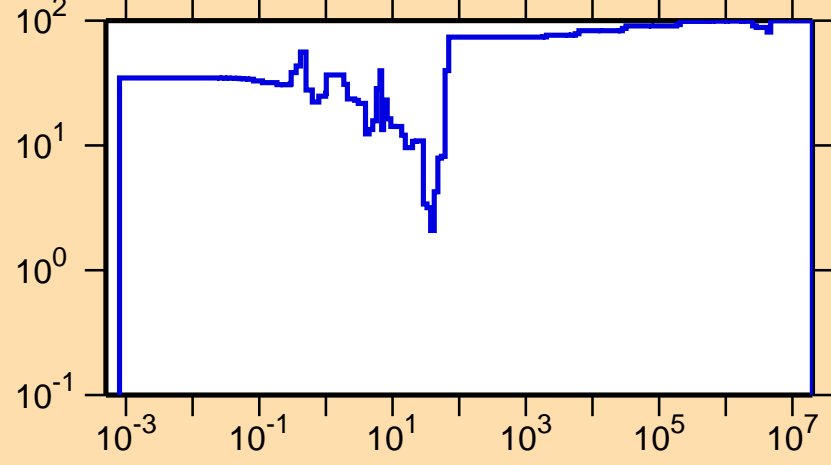
\Delta\sigma/\sigma vs. E for ^{222}\text{Ac}(n,\gamma)
