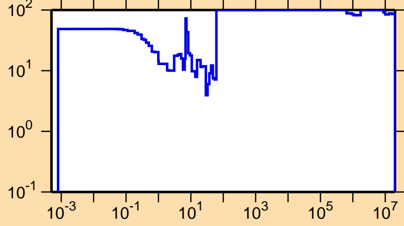
\Delta\sigma/\sigma vs. E for ^{222}\text{Ac}(n,f)
