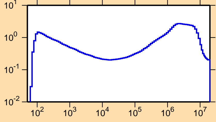
\sigma vs. E for ^{222}\text{Ac}(n,\text{inel.})
