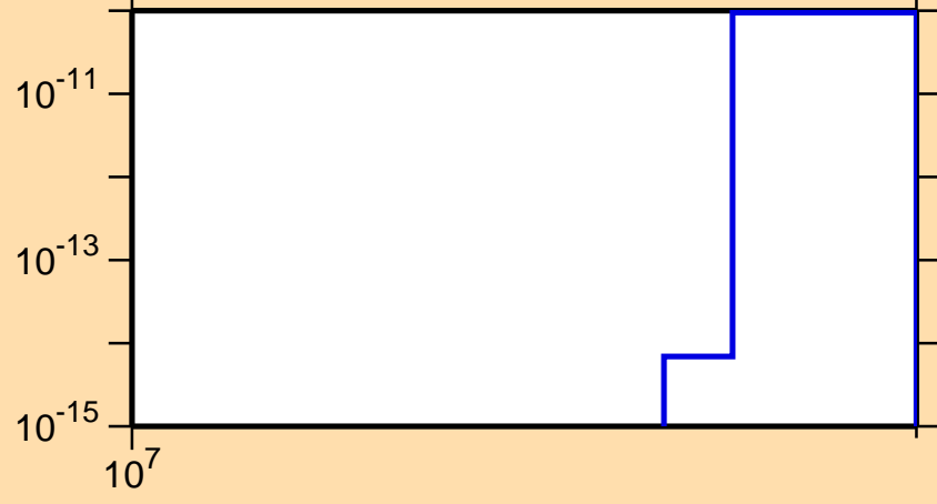
\sigma vs. E for ^{222}\text{Ac}(\text{mt } 11)
