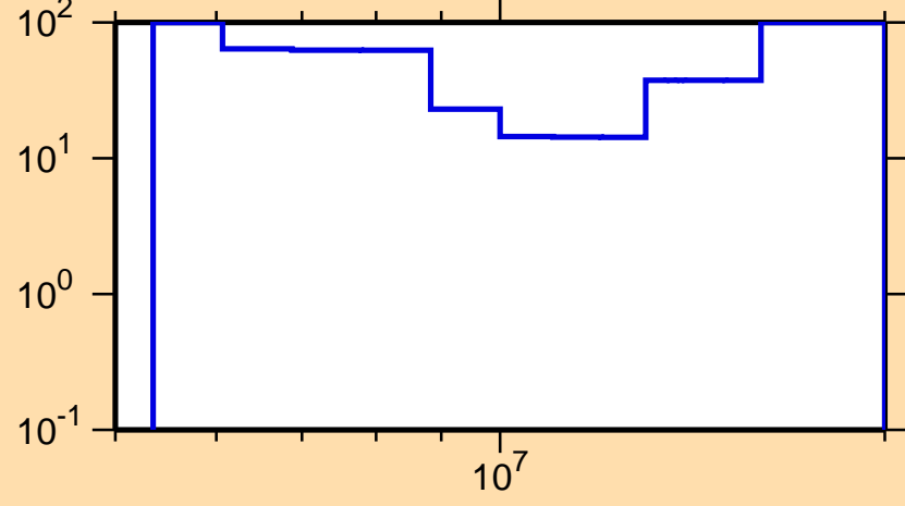
\Delta\sigma/\sigma vs. E for ^{222}\text{Ac}(n,2n)
