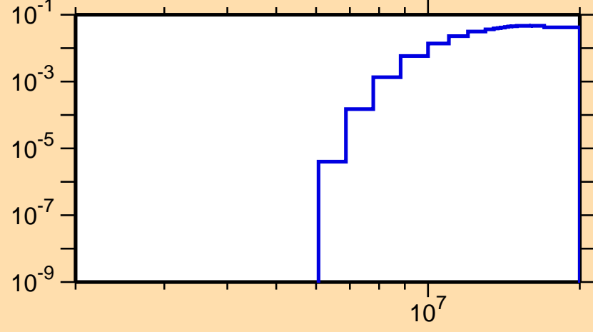
\sigma vs. E for ^{222}\text{Ac}(n,2n\alpha)
