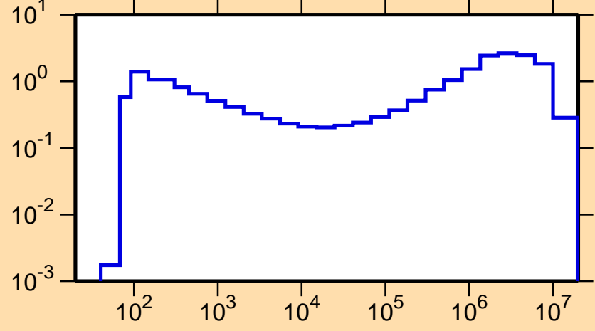
\sigma vs. E for ^{222}\text{Ac}(n,\text{inel.})
