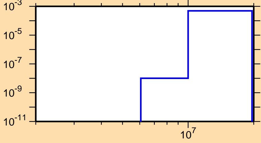
\sigma vs. E for ^{222}\text{Ac}(n,t)
