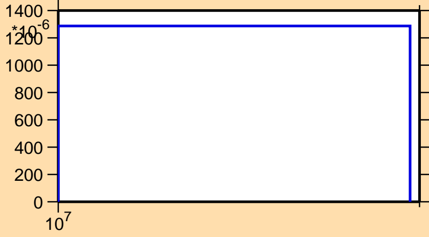
\sigma vs. E for ^{222}\text{Ac}(n,3n\alpha)
