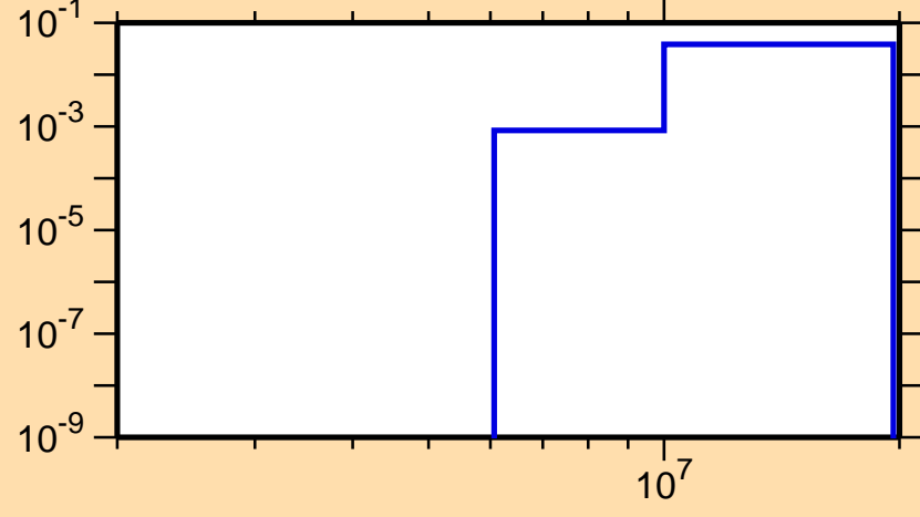
\sigma vs. E for ^{222}\text{Ac}(n,2n\alpha)
