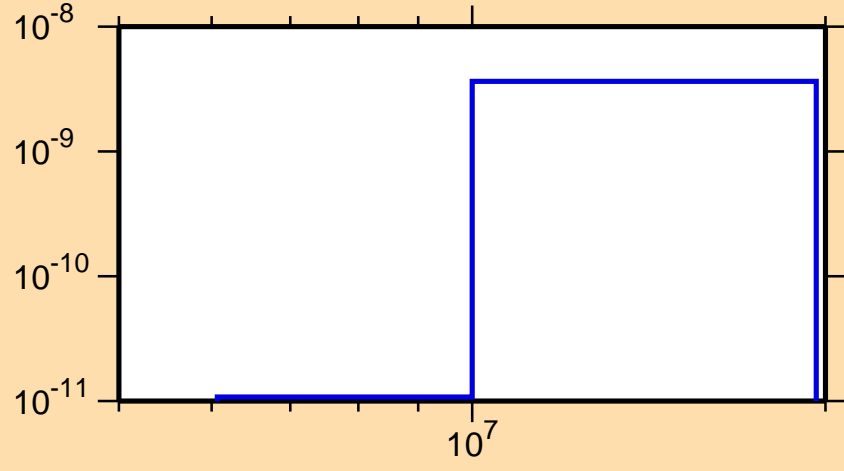
\sigma vs. E for ^{222}\text{Ac}(n,p\alpha)
