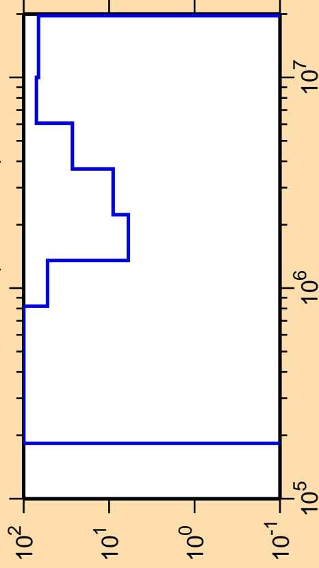
\Delta\sigma/\sigma vs. E for ^{222}\text{Ac}(n,\text{ncont.})
