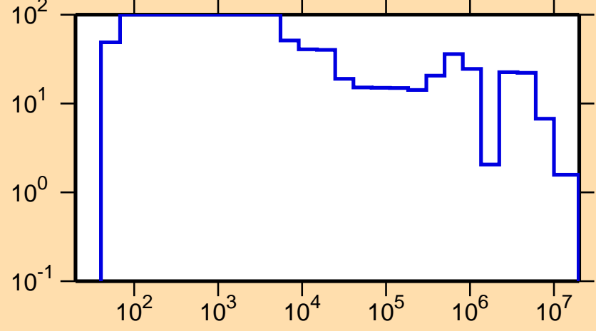
\Delta\sigma/\sigma vs. E for ^{222}\text{Ac}(n,\text{tot.})
