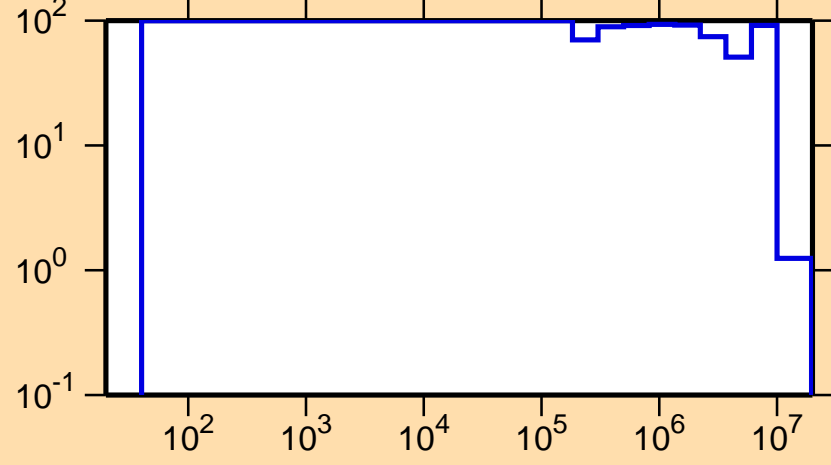
\Delta\sigma/\sigma vs. E for ^{222}\text{Ac}(n,n_1)
