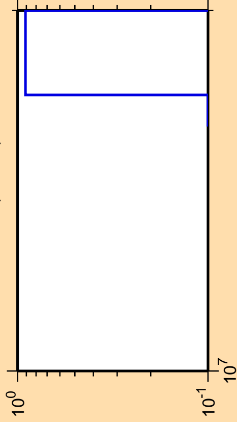
\Delta\sigma/\sigma vs. E for ^{223}\text{Ac}(\text{mt } 34)
