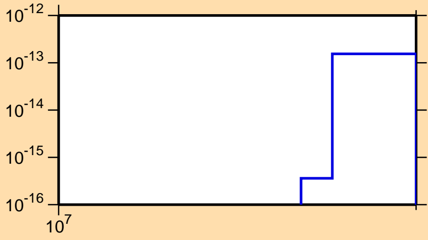
\sigma vs. E for ^{223}\text{Ac}(\text{mt } 34)
