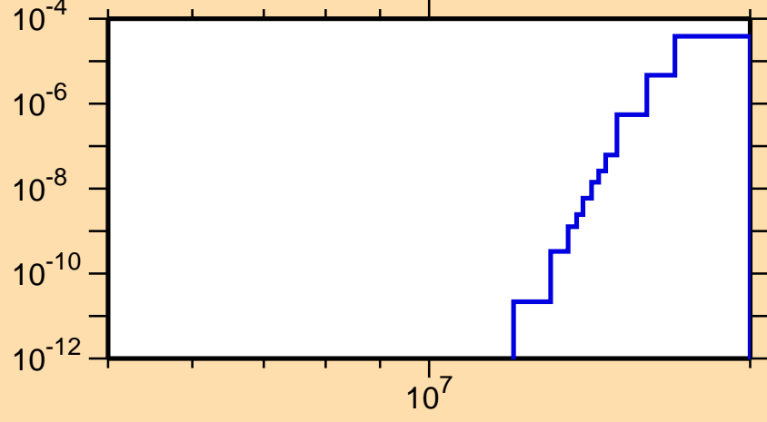
\sigma vs. E for ^{223}\text{Ac}(n,nt)
