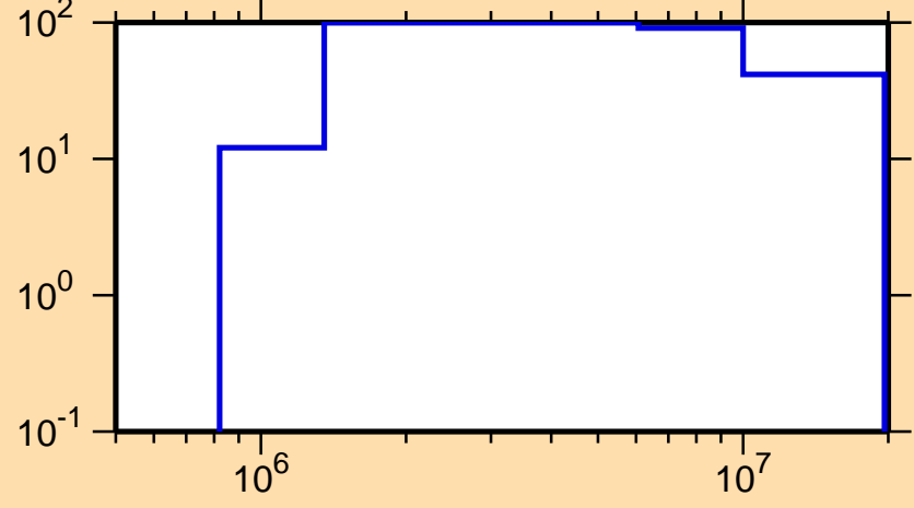
\Delta\sigma/\sigma vs. E for ^{223}\text{Ac}(n,p)
