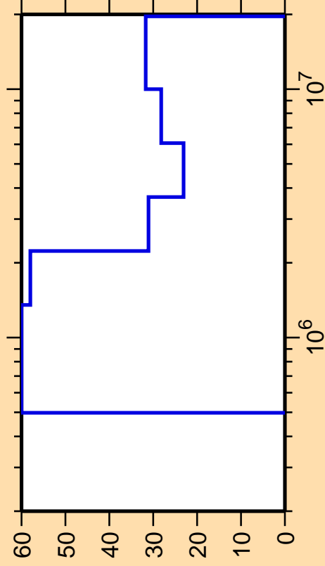
\Delta\sigma/\sigma vs. E for ^{223}\text{Ac}(n,\text{ncont.})
