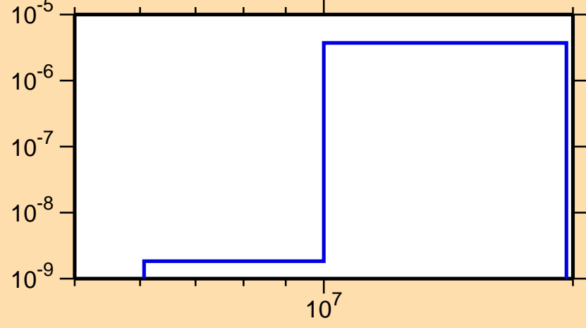
\sigma vs. E for ^{223}\text{Ac}(n,2n\alpha)
