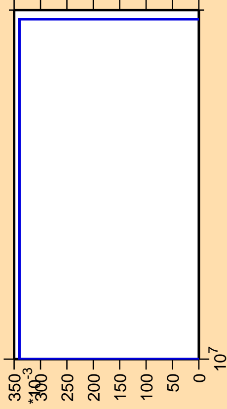
\Delta\sigma/\sigma vs. E for ^{223}\text{Ac} (mt 11)
