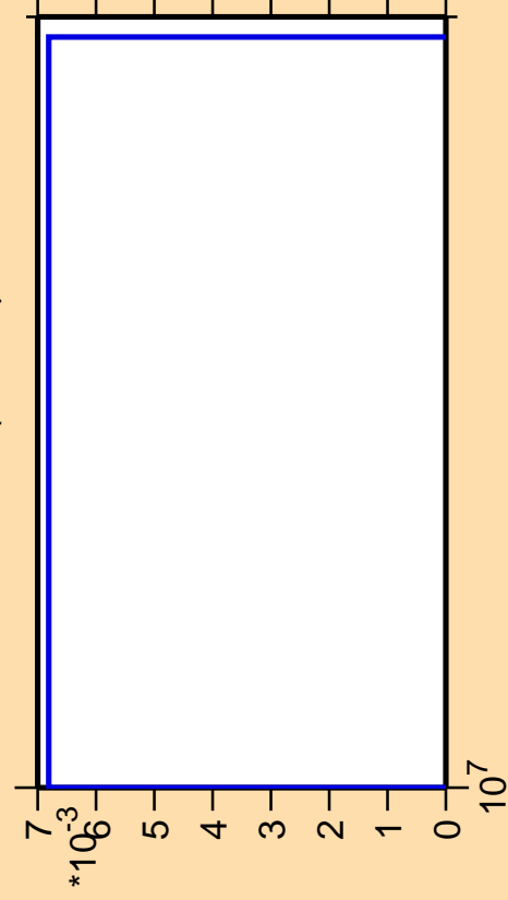
\Delta\sigma/\sigma vs. E for ^{223}\text{Ac} (mt 34)
