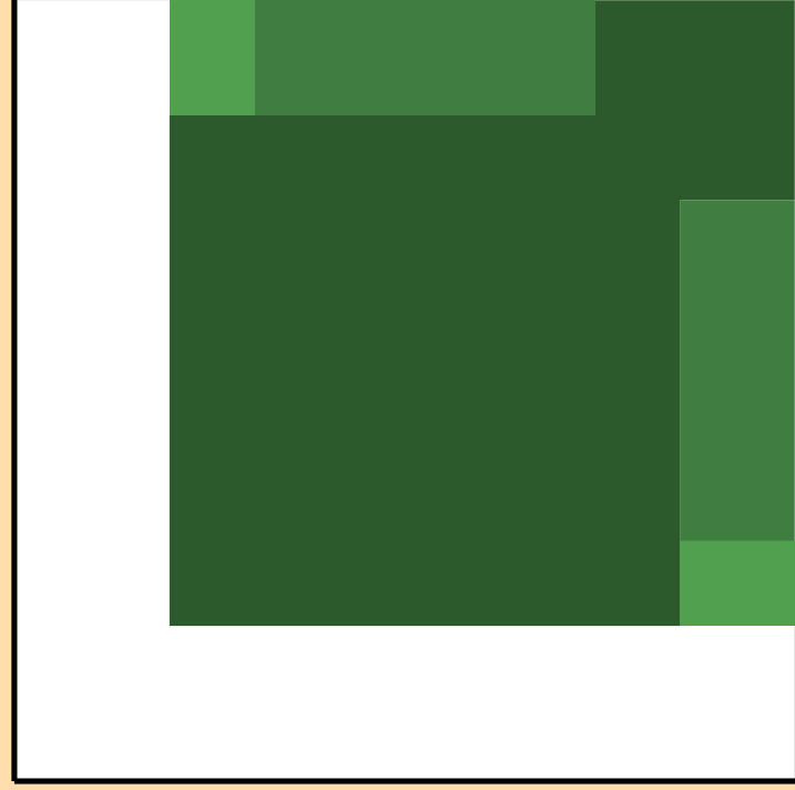
\sigma vs. E for ^{223}\text{Ac}(n,n\text{cont.})
