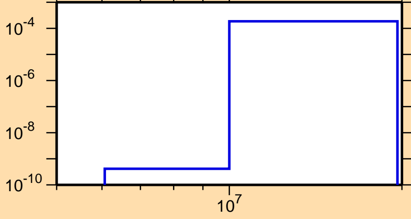
\sigma vs. E for ^{223}\text{Ac}(n,t)
