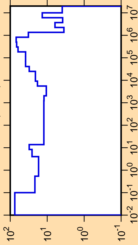
\Delta\sigma/\sigma vs. E for ^{223}\text{Ac}(n,\text{tot.})
