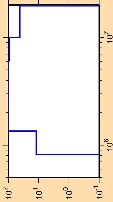
\Delta\sigma/\sigma vs. E for ^{223}\text{Ac}(n,p)
