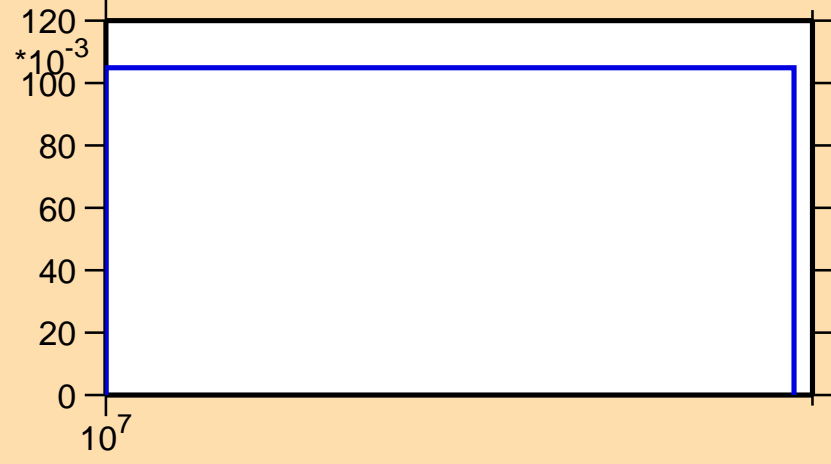
\sigma vs. E for ^{223}\text{Ac}(n,3n)
