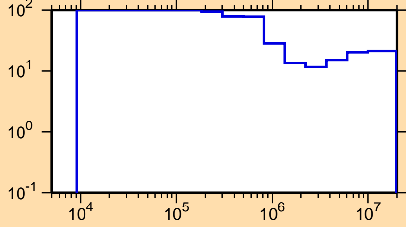
\Delta\sigma/\sigma vs. E for ^{223}\text{Ac}(n,\text{inel.})
