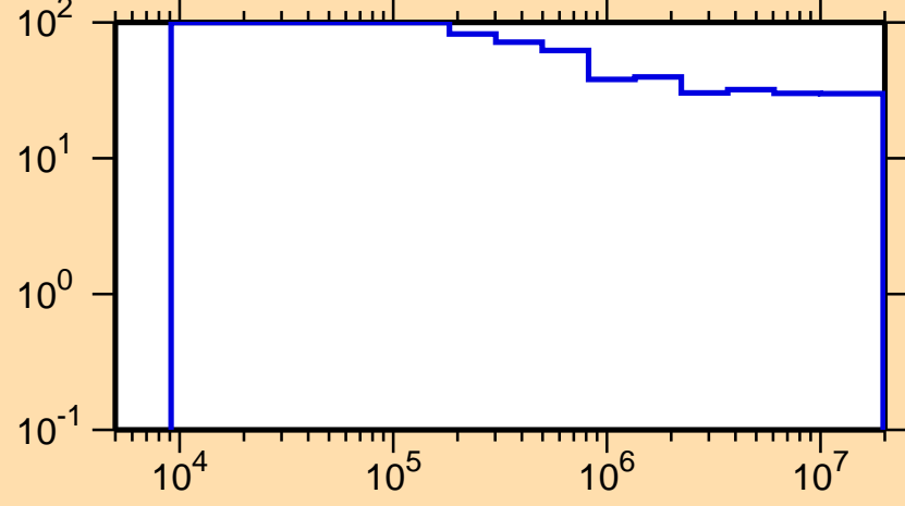
\Delta\sigma/\sigma vs. E for ^{223}\text{Ac}(n,n_1)
