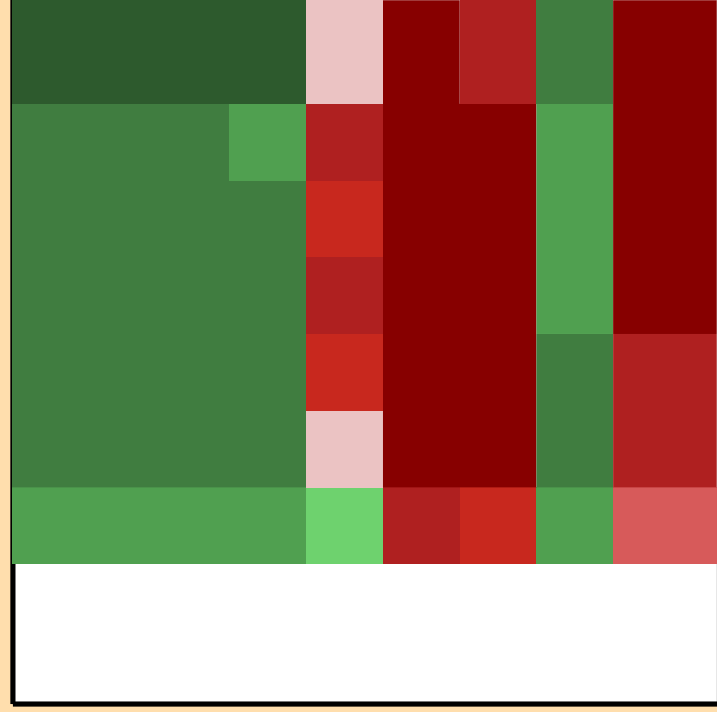
\Delta\sigma/\sigma vs. E for ^{223}\text{Ac}(n,\text{el.})
