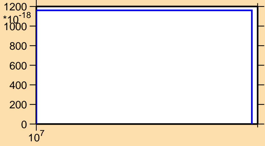
\sigma vs. E for ^{223}\text{Ac} (mt 34)
