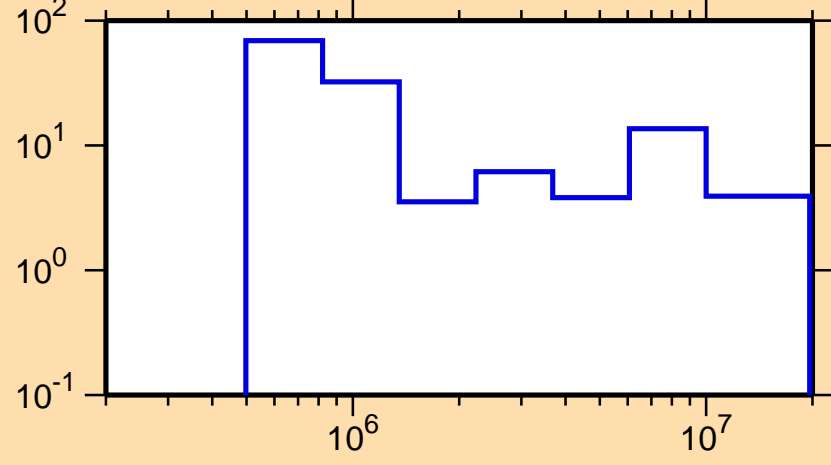
\Delta\sigma/\sigma vs. E for ^{223}\text{Ac}(n,\text{tot.})
