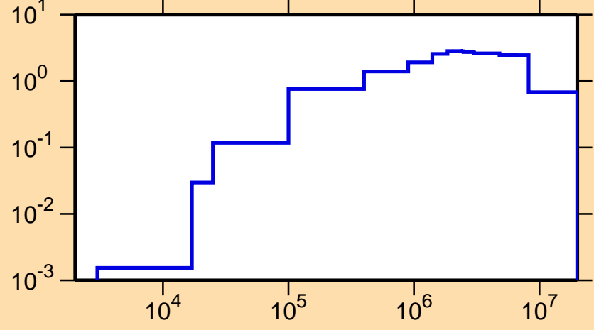
\sigma vs. E for ^{223}\text{Ac}(n,\text{inel.})
