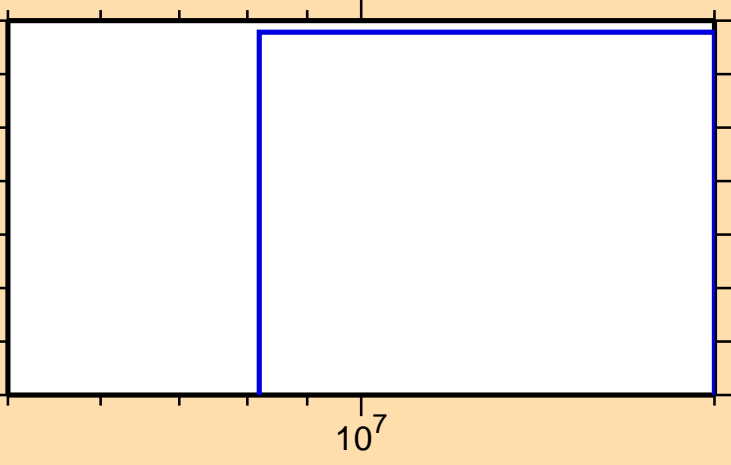
\sigma vs. E for ^{223}\text{Ac}(n,3n\alpha)
