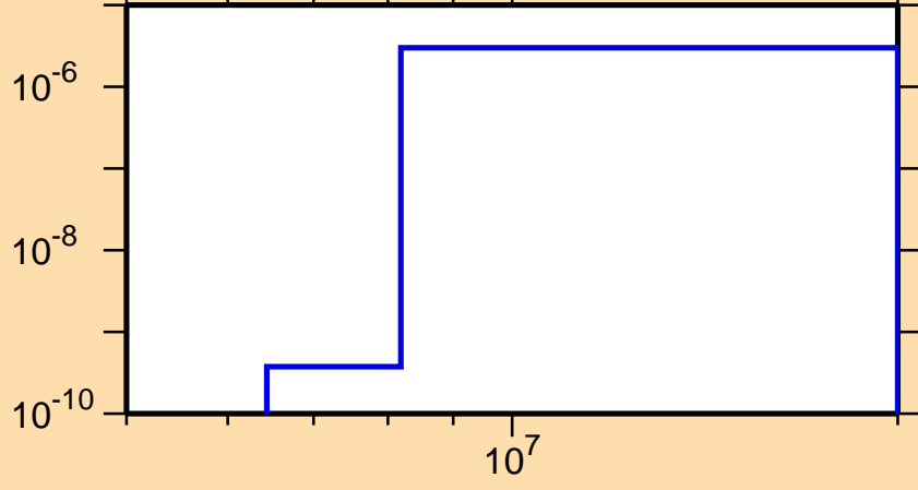
\sigma vs. E for ^{223}\text{Ac}(n,2n\alpha)
