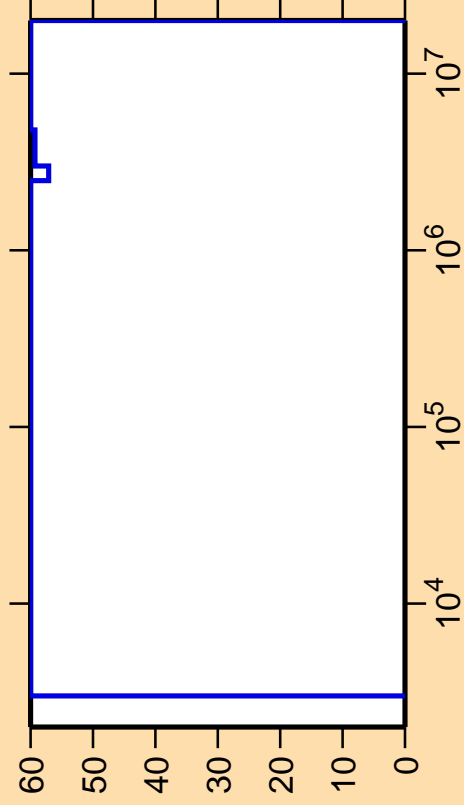
\Delta\sigma/\sigma vs. E for ^{223}\text{Ac}(n,\gamma)
