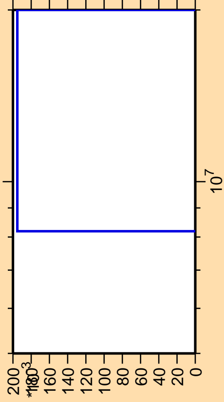
\Delta\sigma/\sigma vs. E for ^{223}\text{Ac}(\text{mt } 42)
