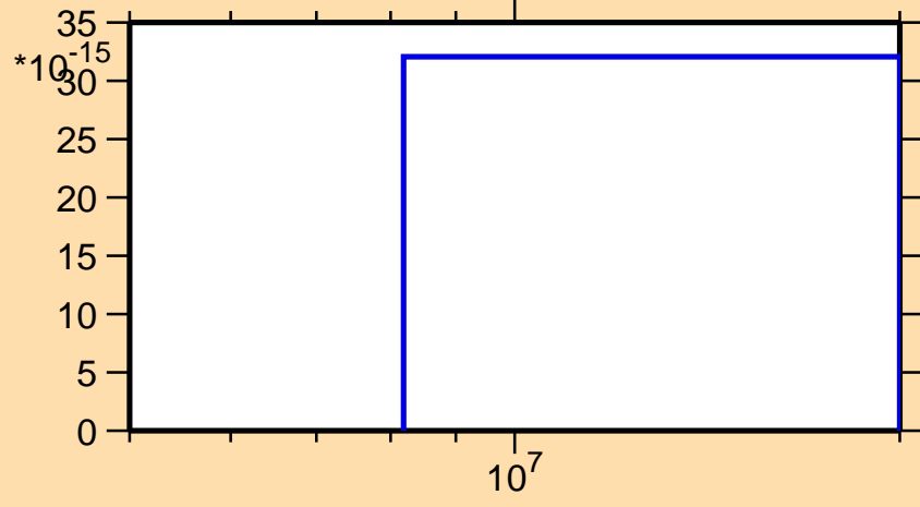
\sigma vs. E for ^{223}\text{Ac}(\text{mt } 42)
