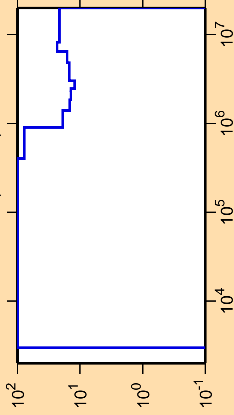
\Delta\sigma/\sigma vs. E for ^{223}\text{Ac}(n,\text{inel.})
