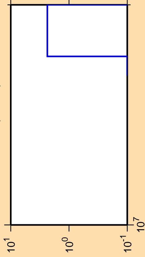
\Delta\sigma/\sigma vs. E for ^{224}\text{Ac}(\text{mt } 42)
