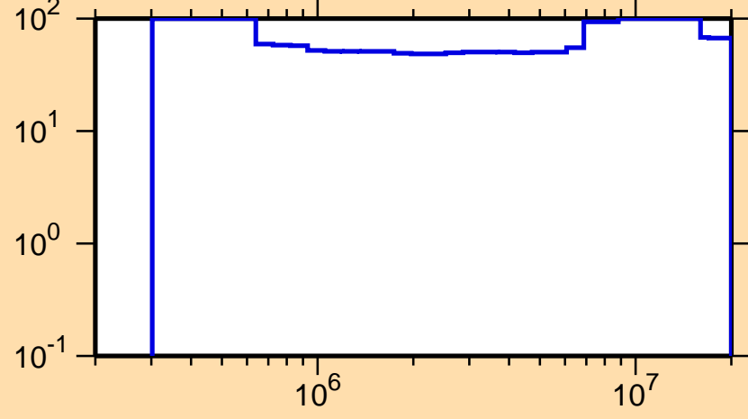
\Delta\sigma/\sigma vs. E for ^{224}\text{Ac}(n,n\text{cont.})
