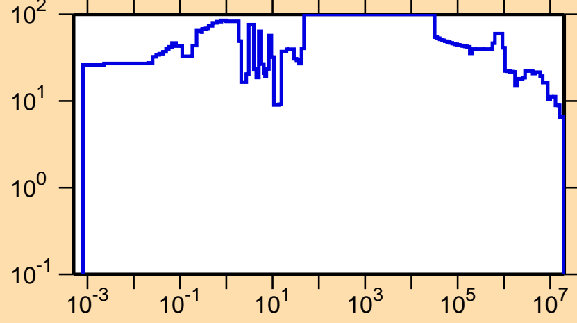
\Delta\sigma/\sigma vs. E for ^{224}\text{Ac}(n,\text{tot.})
