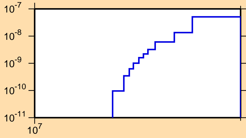
\sigma vs. E for ^{224}\text{Ac}(n,3n\alpha)
