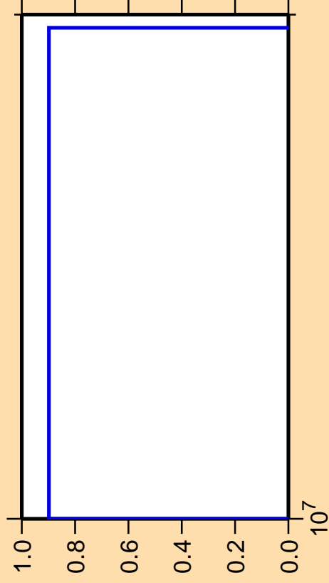
\Delta\sigma/\sigma vs. E for ^{224}\text{Ac} (mt 45)
