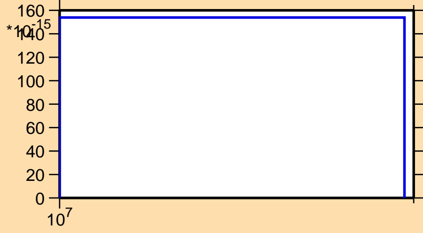
\sigma vs. E for ^{224}\text{Ac} (mt 45)
