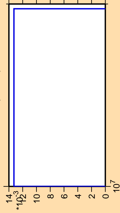
\Delta\sigma/\sigma vs. E for ^{224}\text{Ac} (mt 42)
