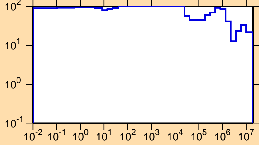
\Delta\sigma/\sigma vs. E for ^{224}\text{Ac}(n,\text{el.})
