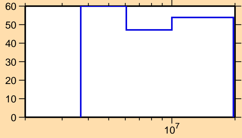
\Delta\sigma/\sigma vs. E for ^{224}\text{Ac}(n,2n)
