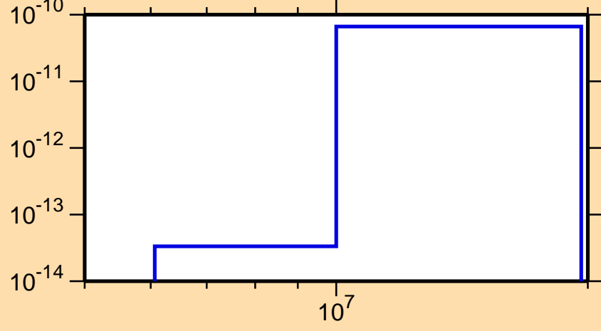
\sigma vs. E for ^{224}\text{Ac}(n,p\alpha)
