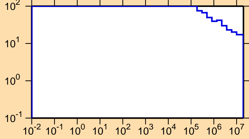
\Delta\sigma/\sigma vs. E for ^{224}\text{Ac}(n,\text{nonel.})
