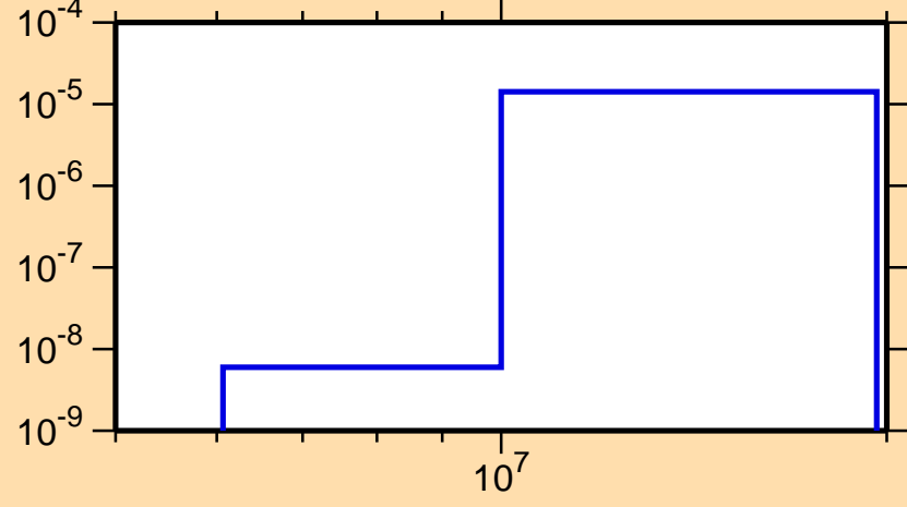
\sigma vs. E for ^{224}\text{Ac}(n,2n\alpha)
