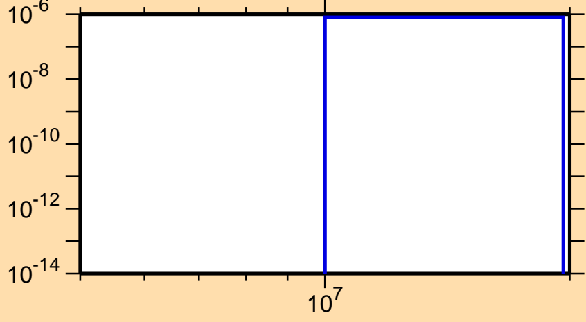
\sigma vs. E for ^{224}\text{Ac}(n,2np)
