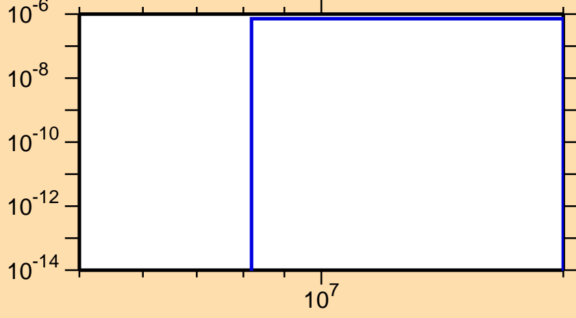
\sigma vs. E for ^{224}\text{Ac}(n,nt)
