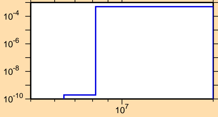
\sigma vs. E for ^{224}\text{Ac}(n,d)
