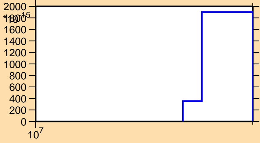
\sigma vs. E for ^{225}\text{Ac} (mt 45)
