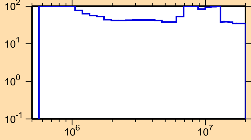
\Delta\sigma/\sigma vs. E for ^{225}\text{Ac}(n,n\text{cont.})
