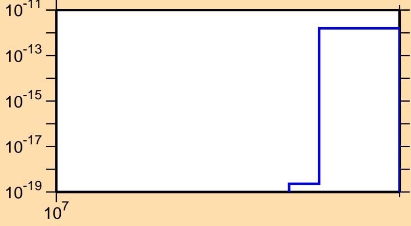
\sigma vs. E for ^{225}\text{Ac} (mt 42)
