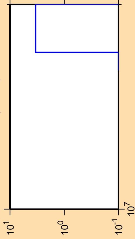
\Delta\sigma/\sigma vs. E for ^{225}\text{Ac} (mt 42)
