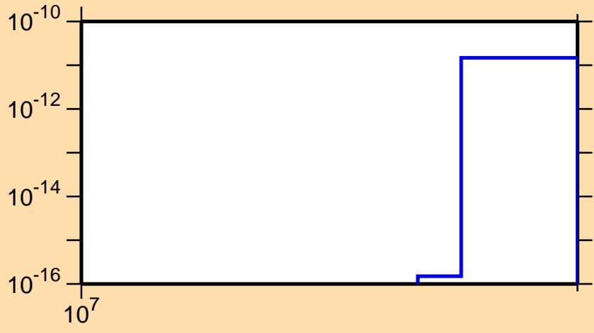
\sigma vs. E for ^{225}\text{Ac} (mt 11)
