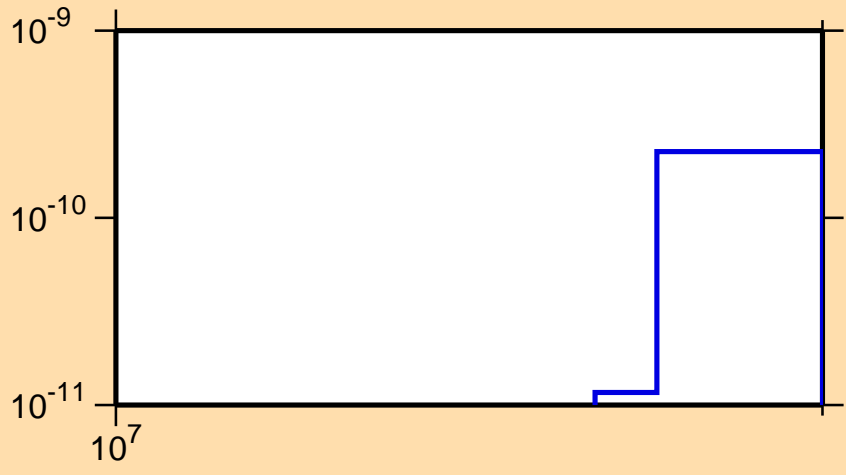
\sigma vs. E for ^{225}\text{Ac}(n,\text{He}3)
