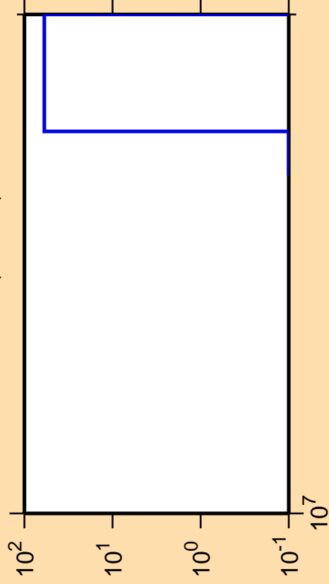
\Delta\sigma/\sigma vs. E for ^{225}\text{Ac} (mt 11)
