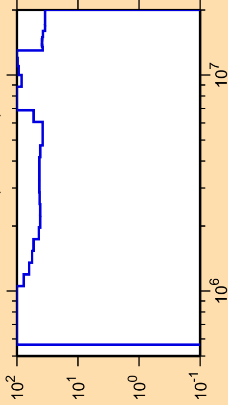
\Delta\sigma/\sigma vs. E for ^{225}\text{Ac}(n,\text{ncont.})
