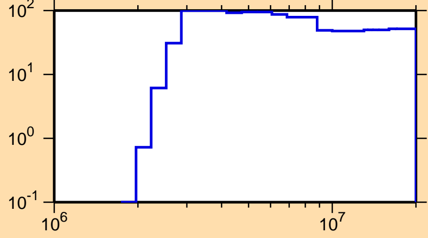
\Delta\sigma/\sigma vs. E for ^{225}\text{Ac}(n,p)
