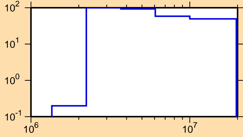
\Delta\sigma/\sigma vs. E for ^{225}\text{Ac}(n,p)
