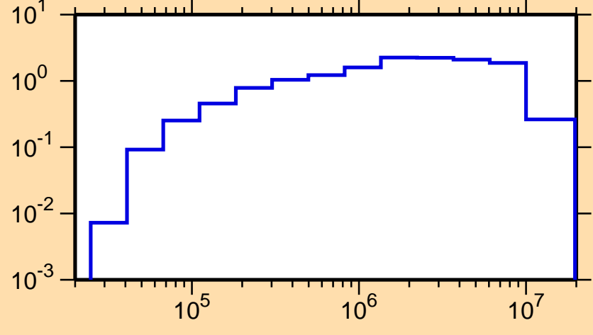
\sigma vs. E for ^{225}\text{Ac}(n,\text{inel.})
