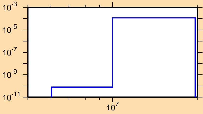
\sigma vs. E for ^{225}\text{Ac}(n,t)
