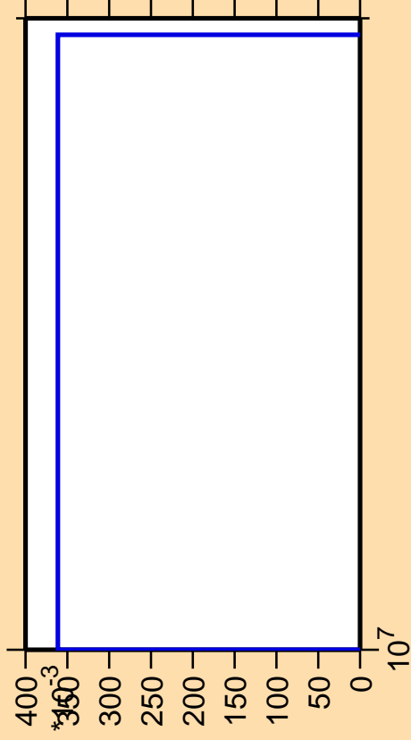
\Delta\sigma/\sigma vs. E for ^{225}\text{Ac} (mt 11)
