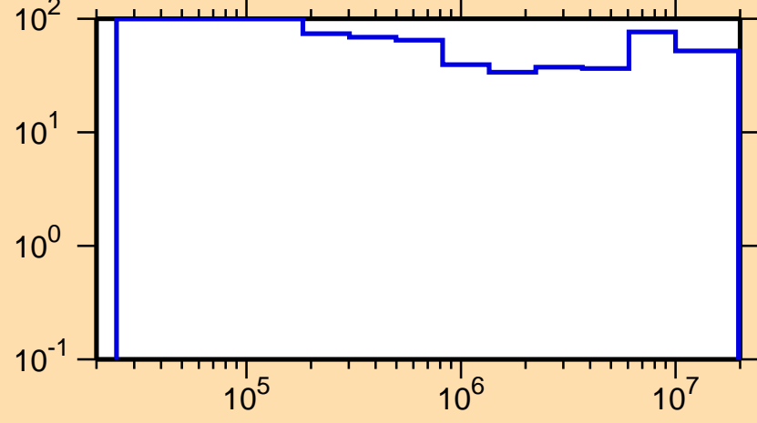
\Delta\sigma/\sigma vs. E for ^{225}\text{Ac}(n,\text{inel.})
