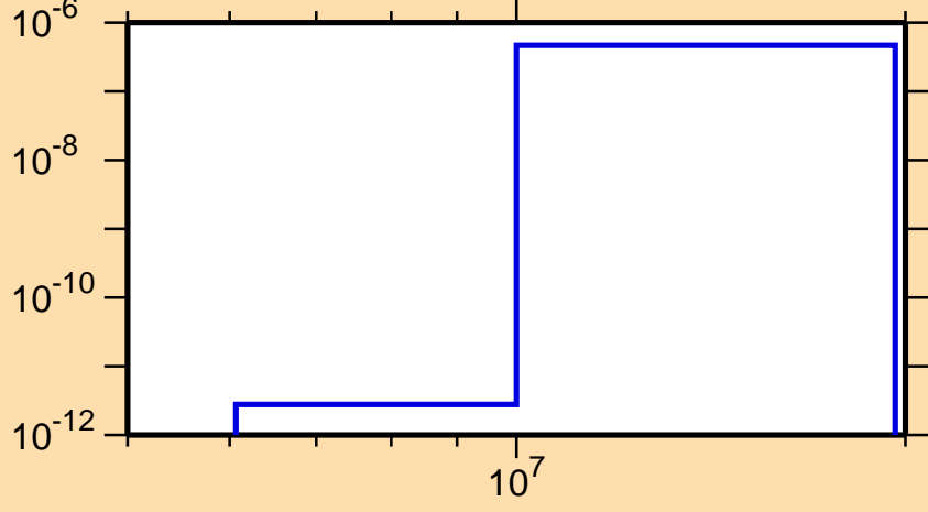
\sigma vs. E for ^{225}\text{Ac}(n,2n\alpha)
