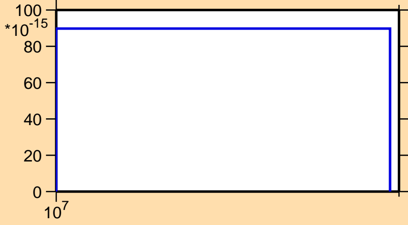
\sigma vs. E for ^{225}\text{Ac} (mt 11)
