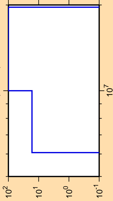
\Delta\sigma/\sigma vs. E for ^{225}\text{Ac}(n,2n\alpha)
