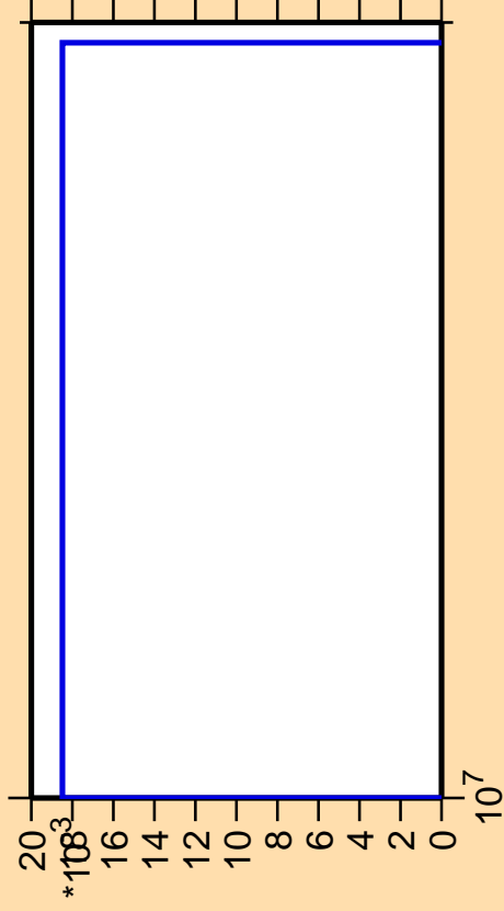
\Delta\sigma/\sigma vs. E for ^{225}\text{Ac} (mt 42)
