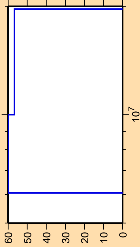
\Delta\sigma/\sigma vs. E for ^{225}\text{Ac}(n,d)
