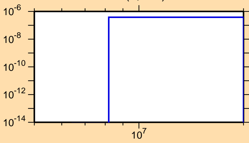
\sigma vs. E for ^{225}\text{Ac}(n,2n\alpha)
