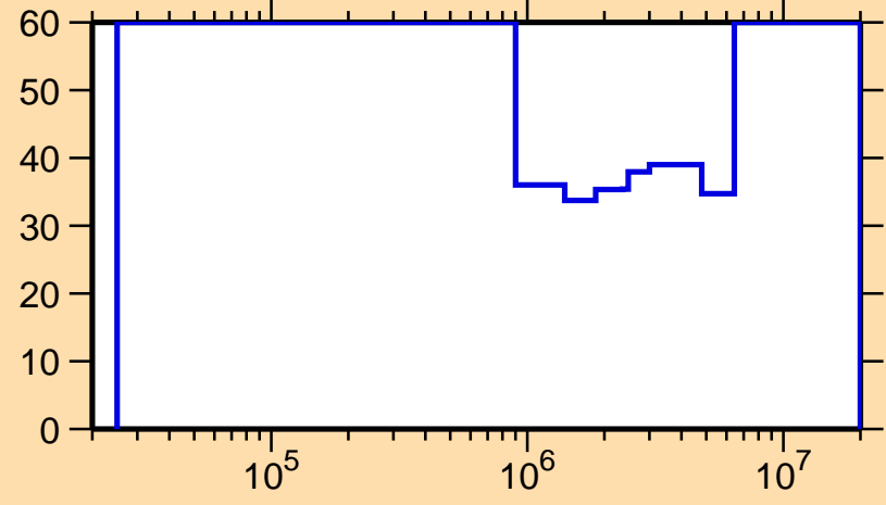
\Delta\sigma/\sigma vs. E for ^{225}\text{Ac}(n,inel.)
