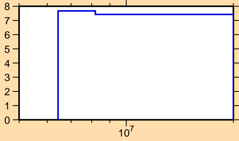
\Delta\sigma/\sigma vs. E for ^{225}\text{Ac}(n,\text{tot.})
