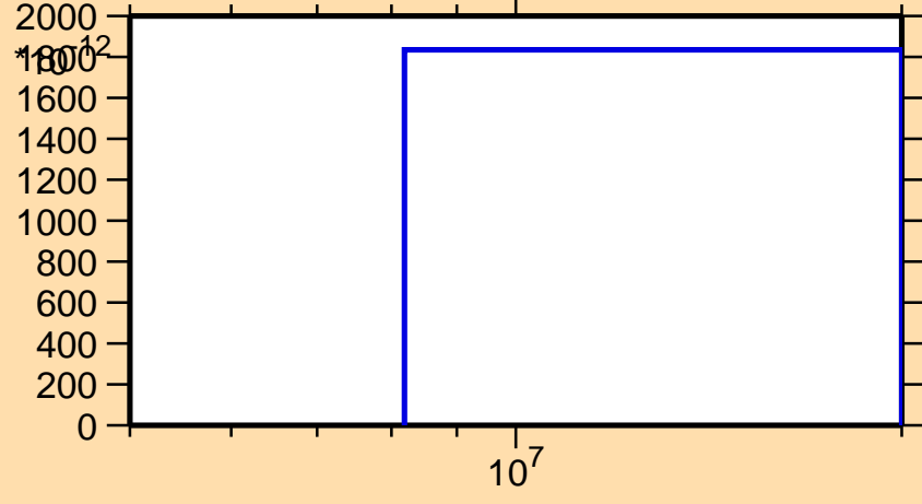
\sigma vs. E for ^{225}\text{Ac}(n,3n\alpha)
