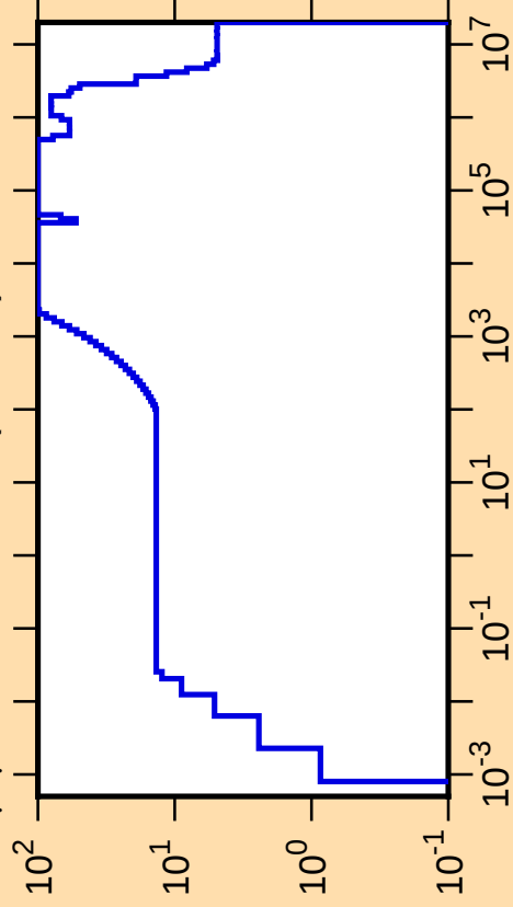
\Delta\mu/\mu vs. E for ^{226}\text{Ac}(\text{mt251})
