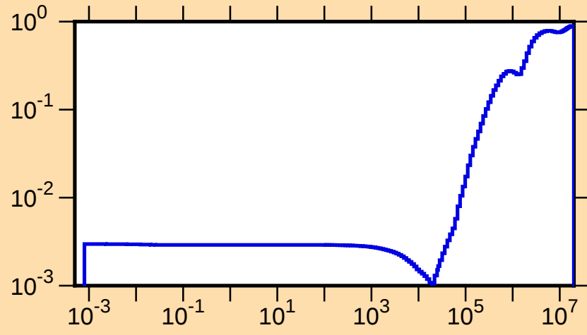
\mu vs. E for ^{226}\text{Ac}(\text{mt251})
