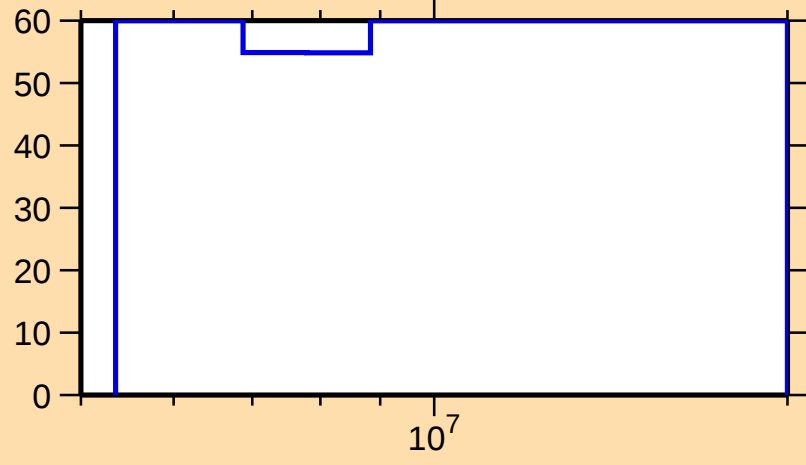
\Delta\sigma/\sigma vs. E for ^{226}\text{Ac}(n,2n)
