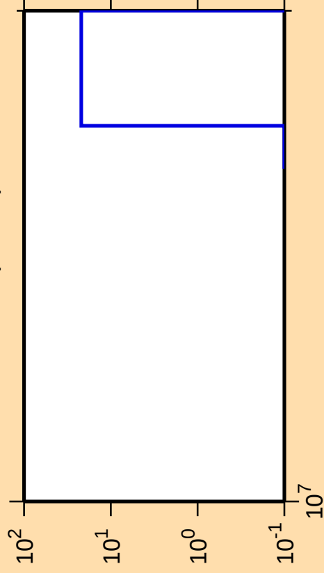
\Delta\sigma/\sigma vs. E for ^{226}\text{Ac}(\text{mt } 11)
