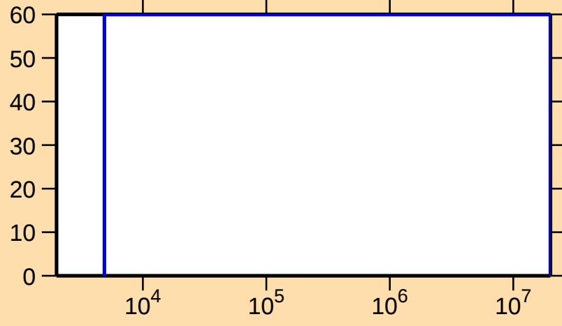
\Delta\sigma/\sigma vs. E for ^{226}\text{Ac}(n,f)
