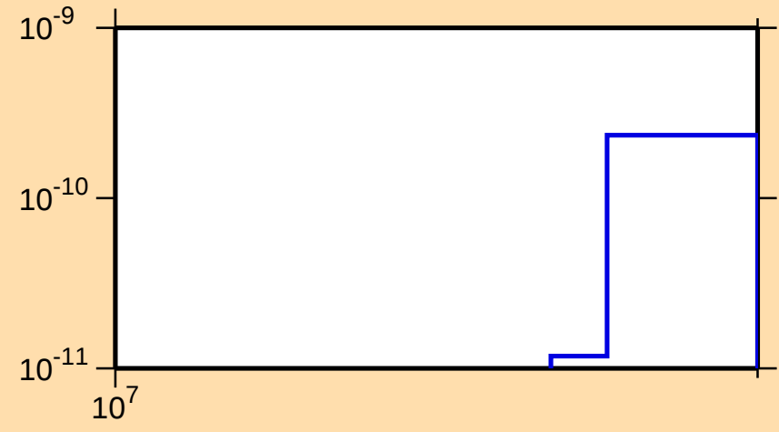
\sigma vs. E for ^{226}\text{Ac}(n,\text{He3})
