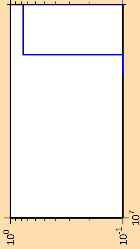
\Delta\sigma/\sigma vs. E for ^{226}\text{Ac}(\text{mt } 42)
