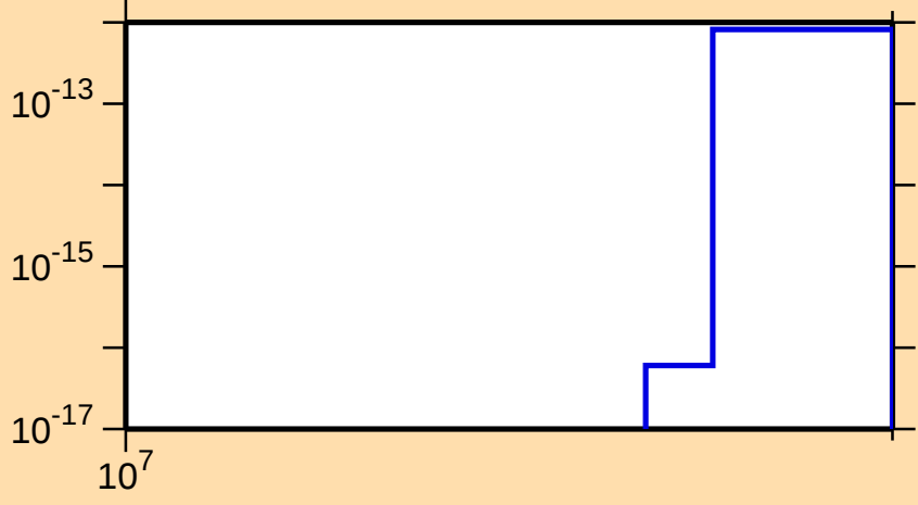
\sigma vs. E for ^{226}\text{Ac}(\text{mt } 42)
