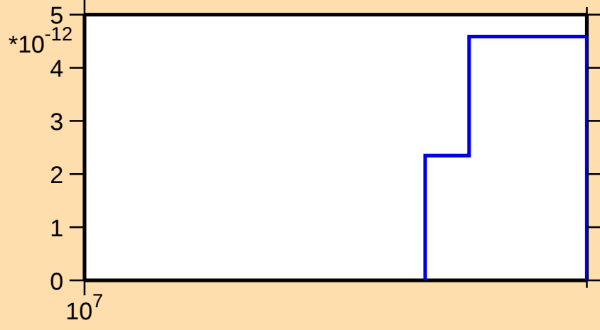
\sigma vs. E for ^{226}\text{Ac}(n,p\alpha)
