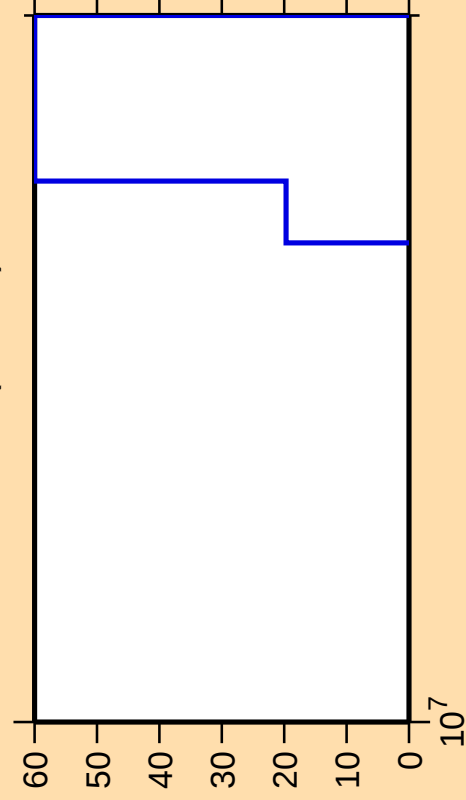
\Delta\sigma/\sigma vs. E for ^{226}\text{Ac}(n,\text{He3})
