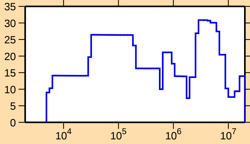
\Delta\sigma/\sigma vs. E for ^{226}\text{Ac}(n,\text{el.})
