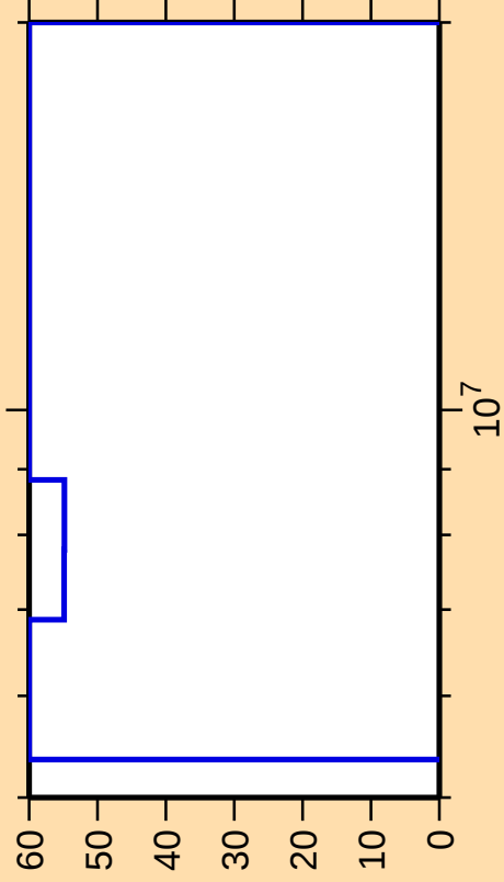
\Delta\sigma/\sigma vs. E for ^{226}\text{Ac}(n,2n)
