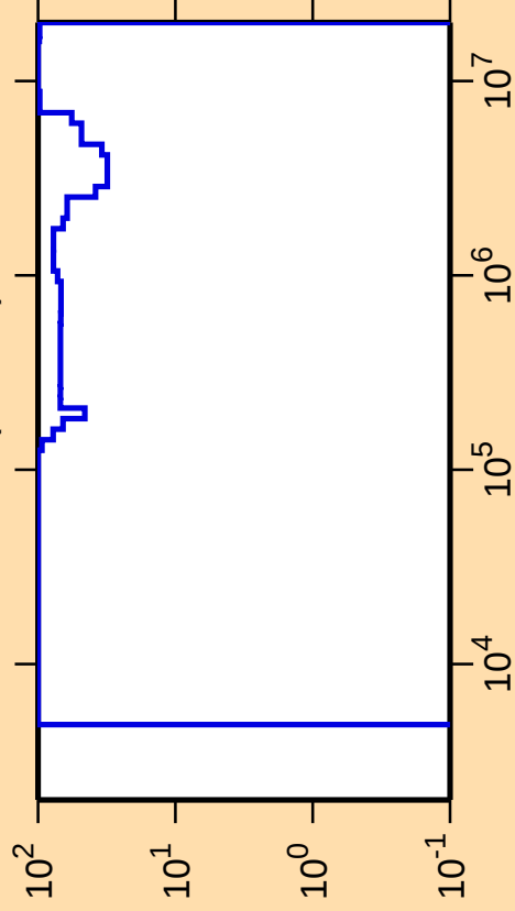
\Delta\sigma/\sigma vs. E for ^{226}\text{Ac}(n,\text{inel.})
