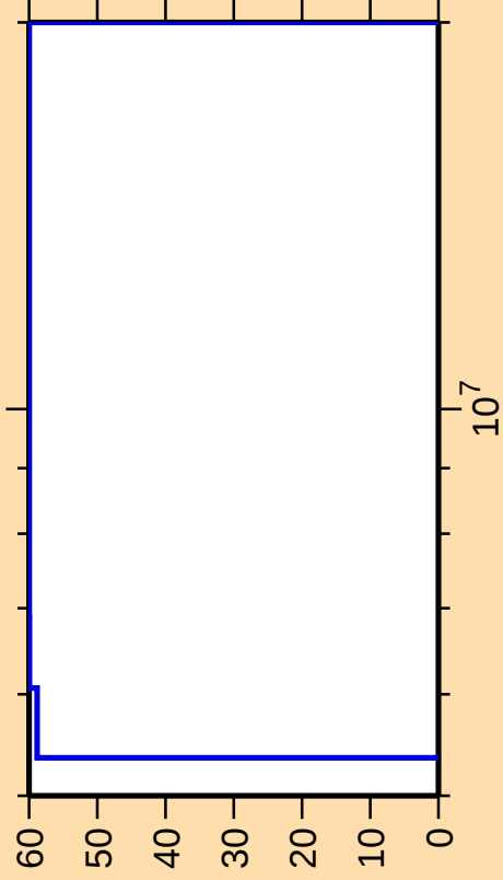
\Delta\sigma/\sigma vs. E for ^{226}\text{Ac}(n,p)
