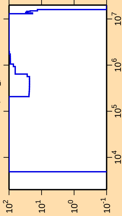
\Delta\sigma/\sigma vs. E for ^{226}\text{Ac}(n,n_1)
