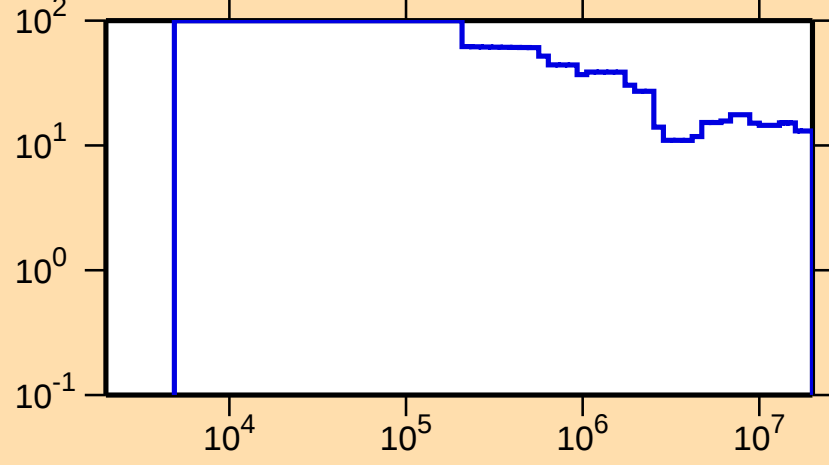
\Delta\sigma/\sigma vs. E for ^{226}\text{Ac}(n,\text{nonel.})
