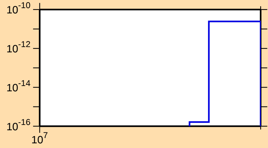
\sigma vs. E for ^{226}\text{Ac}(\text{mt } 11)
