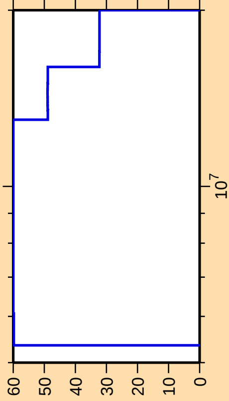
\Delta\sigma/\sigma vs. E for ^{226}\text{Ac}(n,\gamma)
