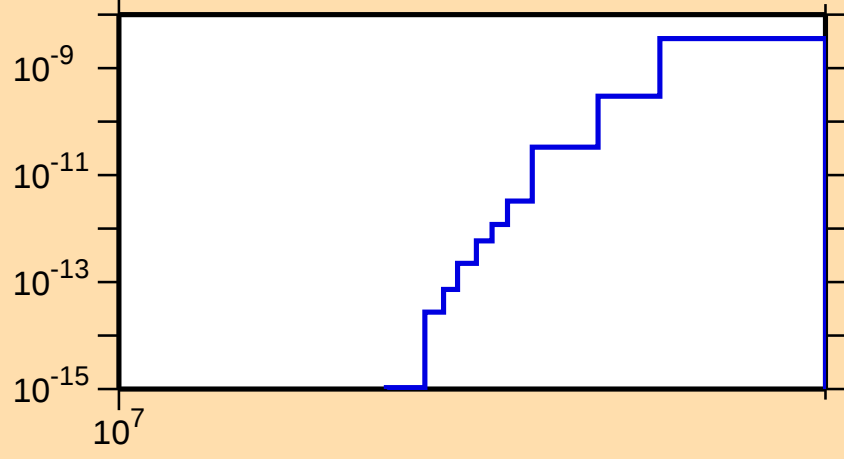
\sigma vs. E for ^{226}\text{Ac}(n,3n\alpha)
