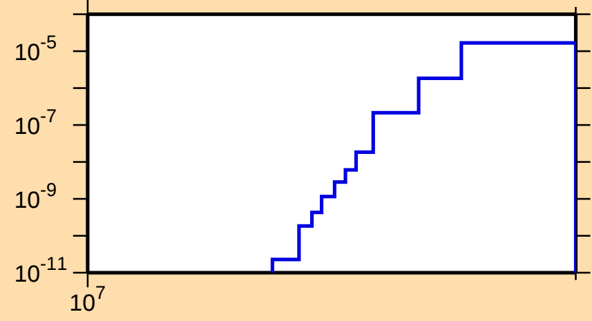
\sigma vs. E for ^{226}\text{Ac}(n,2np)
