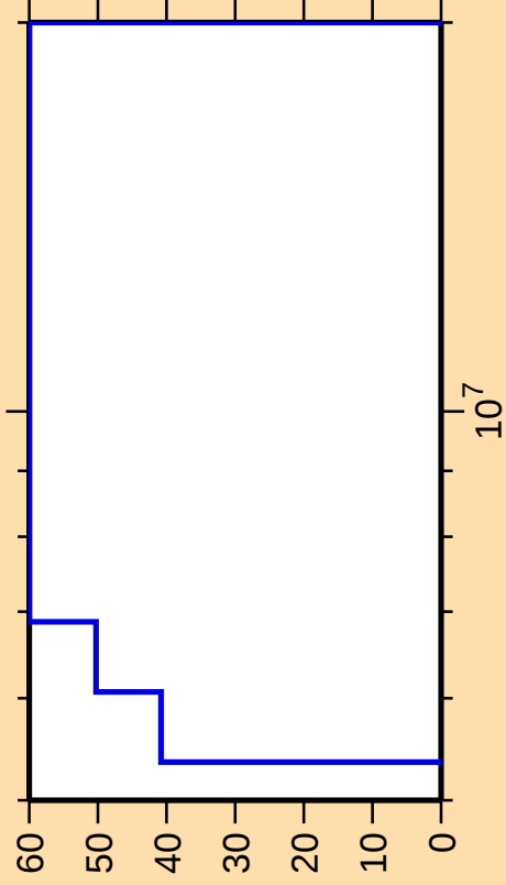
\Delta\sigma/\sigma vs. E for ^{226}\text{Ac}(n,n\text{cont.})
