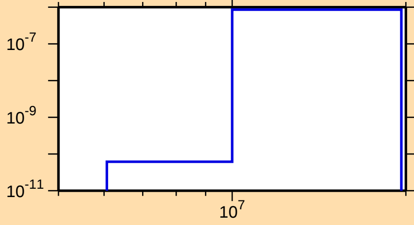
\sigma vs. E for ^{226}\text{Ac}(n,2n\alpha)
