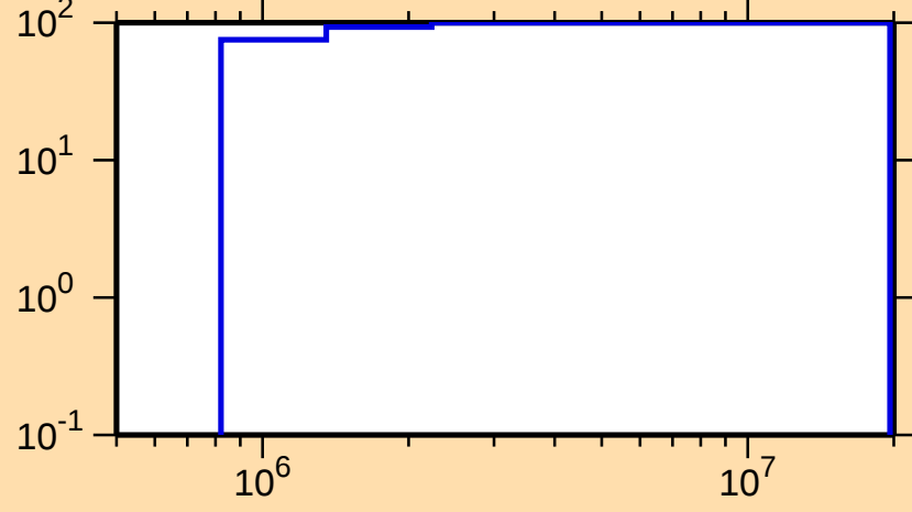
\Delta\sigma/\sigma vs. E for ^{226}\text{Ac}(n,n_1)
