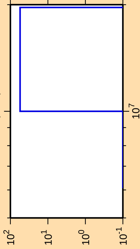
\Delta\sigma/\sigma vs. E for ^{226}\text{Ac}(n,\text{nt})
