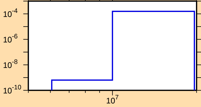
\sigma vs. E for ^{226}\text{Ac}(n,t)
