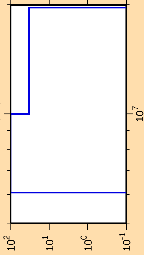
\Delta\sigma/\sigma vs. E for ^{226}\text{Ac}(n,t)
