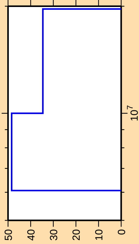
\Delta\sigma/\sigma vs. E for ^{226}\text{Ac}(n,d)
