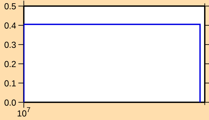
\sigma vs. E for ^{226}\text{Ac}(n,3n)
