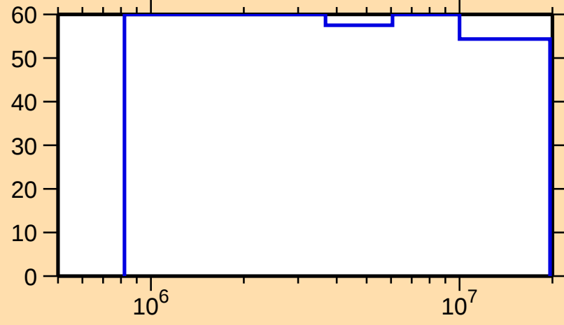
\Delta\sigma/\sigma vs. E for ^{226}\text{Ac}(n,\gamma)
