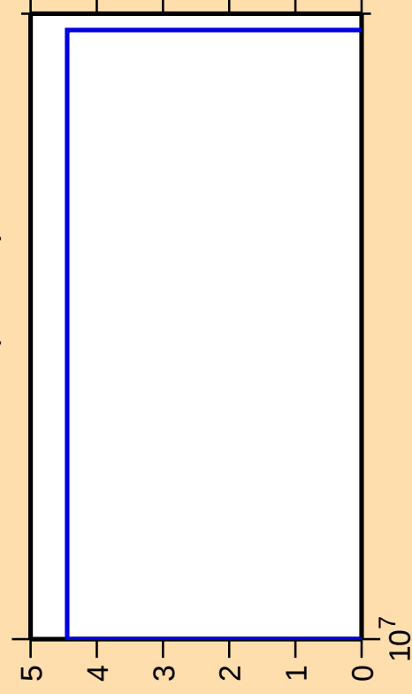
\Delta\sigma/\sigma vs. E for ^{226}\text{Ac}(n,\text{He3})
