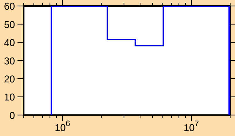
\Delta\sigma/\sigma vs. E for ^{226}\text{Ac}(n,\text{inel.})
