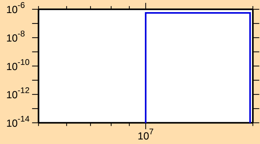
\sigma vs. E for ^{226}\text{Ac}(n,\text{nt})
