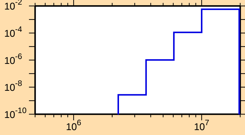
\sigma vs. E for ^{226}\text{Ac}(n,p)
