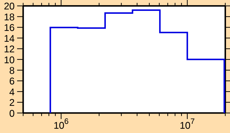
\Delta\sigma/\sigma vs. E for ^{226}\text{Ac}(n,\text{tot.})
