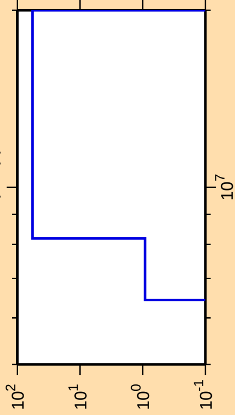
\Delta\sigma/\sigma vs. E for ^{226}\text{Ac}(n,np)
