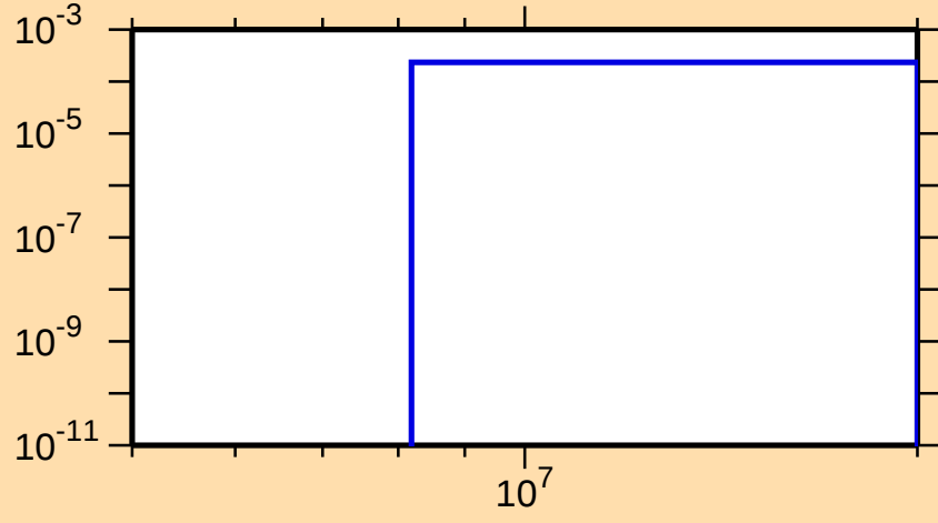
\sigma vs. E for ^{226}\text{Ac}(n,np)
