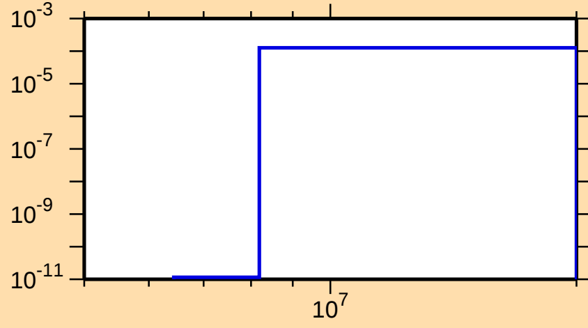
\sigma vs. E for ^{226}\text{Ac}(n,t)
